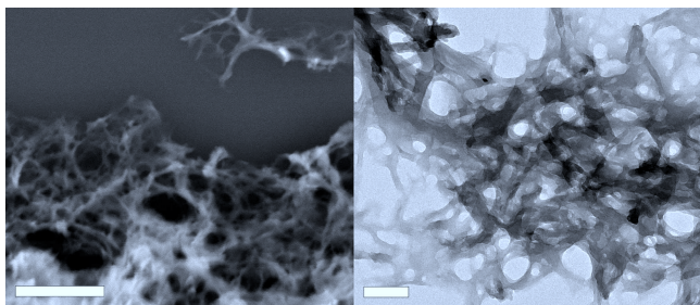
Figure 2. SEM and TEM images of the obtained PTI. The ribbonlike fragments arrange in loose networks with a high porosity. The scale bars in the SEM and TEM images are 500 and 100 nm, respectively.
