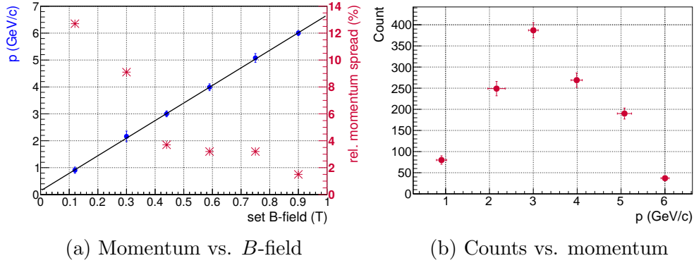
Figure 36: (a): The particle momentum of the simulated test beam as a function of the magnetic field strength of the dipole magnet of TB21. The plot shows the mean momenta for corresponding magnetic field strengths. (b): The simulated particle counts in area of TB21 after the final collimation with respect to the electron momentum. This assumes a fixed DESY II beam energy of 6.3 GeV. The non-constant DESY II beam intensity as well as the time structure given by the sinusoidal DESY II magnet cycle (see Sec. 3) are not considered in this simulation.
