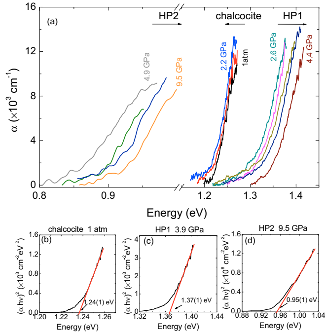
FIG. 10. (a) Absorption spectra of \text{Cu}_2\text{S} at different pressures on pressure release from 9.5 GPa to ambient pressure. The energy dependence of (h\nu\alpha)^2 and the extrapolation of the linear portion intercepting the energy axis are shown for (b) \alpha -chalcocite at 1 atm, (c) HP1 at 3.9(2) GPa, and (d) HP2 at 9.5(5) GPa.
