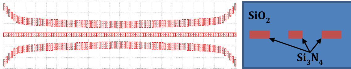
Figure 11. Top view of mask layout for a double-chirped grating where the coupling is adiabatically switched on by bringing the grating sections slowly closer to the main waveguide where the guided light comes in [16].
