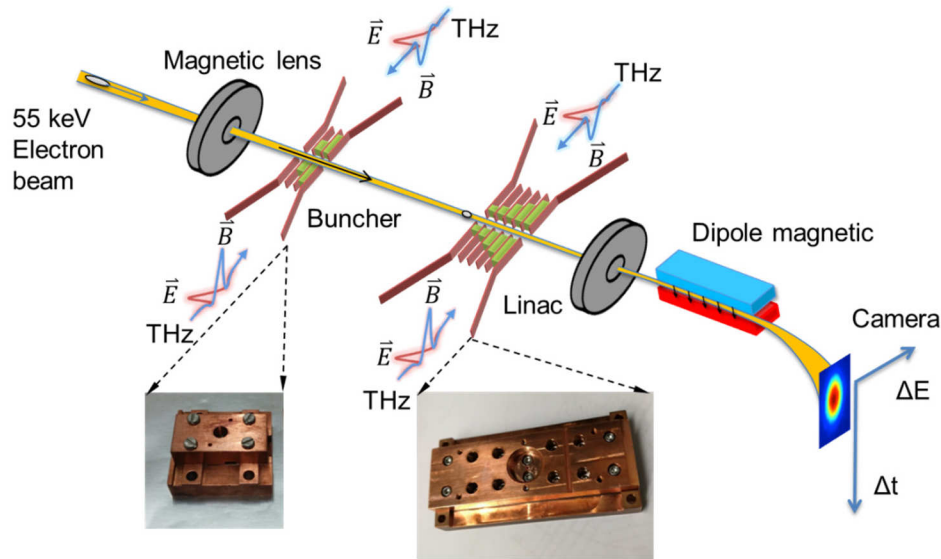
Figure 1: Acceleration of an electron bunch from a 55 keV DC-gun using a STEAM-Buncher and STEAM-LINAC followed by a dipole magnet for energy measurement on a MCP; Inset: STEAM Buncher (left) and STEAM LINAC (right).
