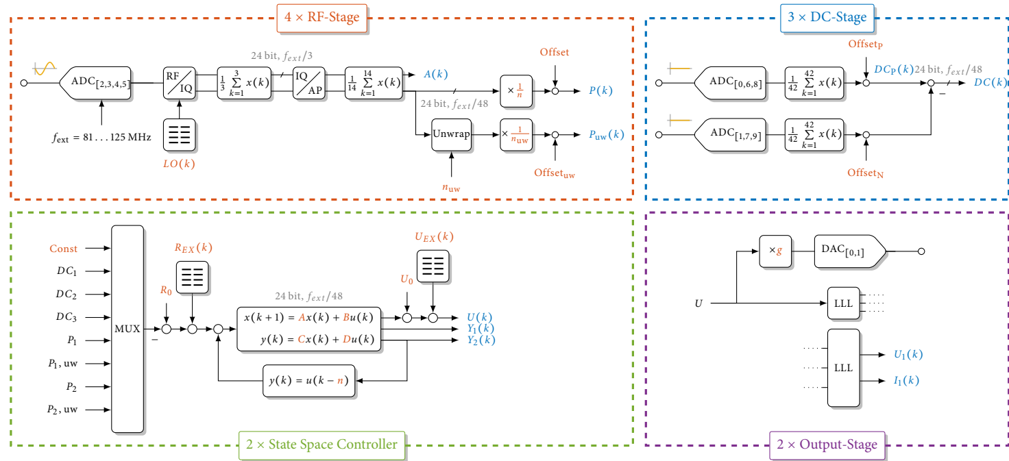
Figure B.2: Simplified block diagram of the MLO firmware.
