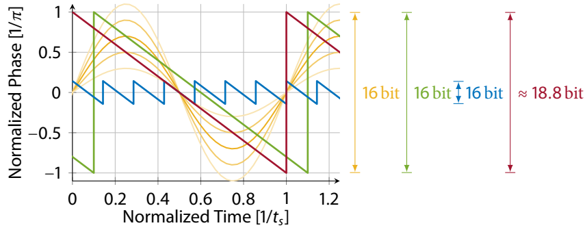
Figure 4.25: Normalized plot of detection scheme with the real phase difference (—), the direct signal (—), and the signal of the 7th harmonic (—).
