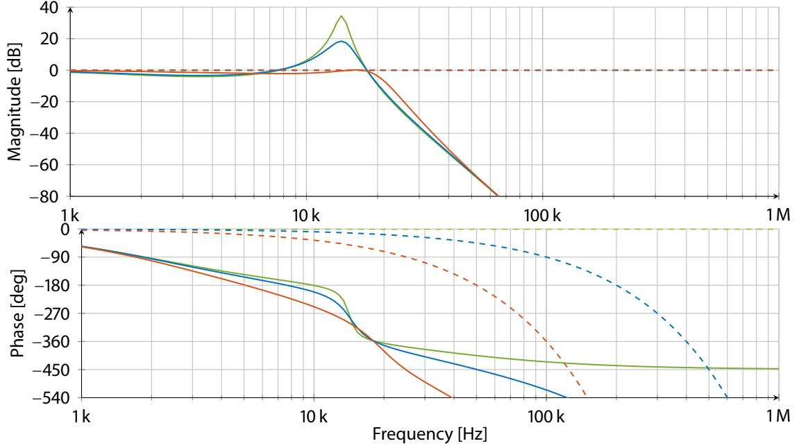
Figure 5.44: Bode diagram of the closed loop using a PI controller without (—) with an additional time delay of 2.5 \mu\text{s} (—) and 10 \mu\text{s} (—) with the corresponding open loop transfer functions of the time delays (---) and (---) and the unit gain (---).
