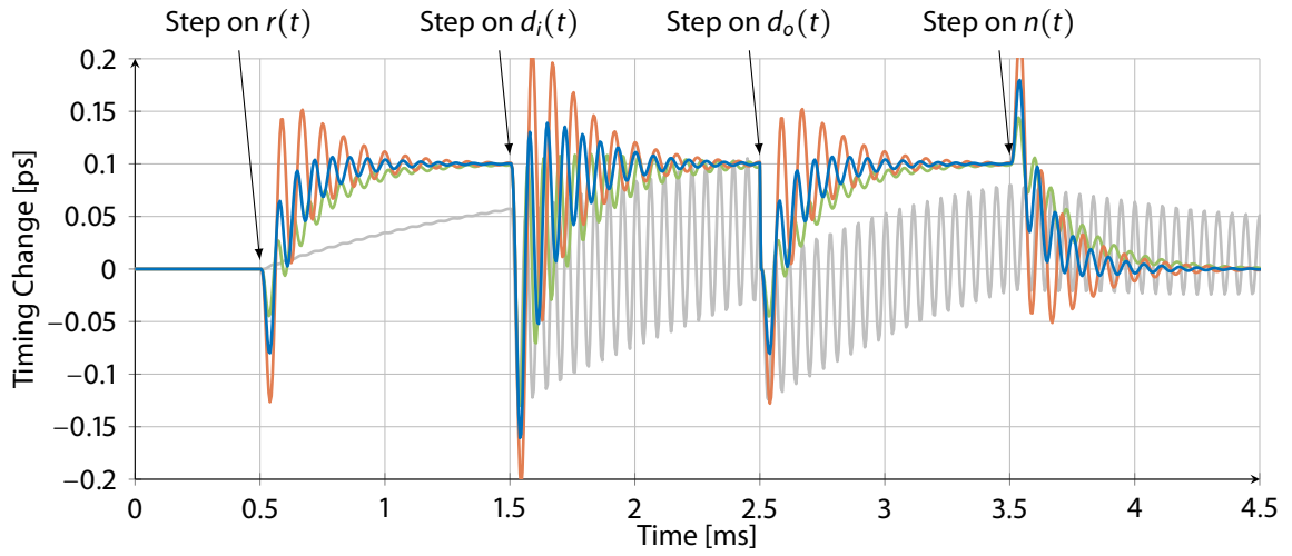
Figure 5.33: Simulated response of the heuristically tuned PI controller (—) and the previous used integral controller (—) to the test sequence with nominal plant. Furthermore, the assumed plant variation are shown by an increased gain (—), a decreased gain (—) gain.
