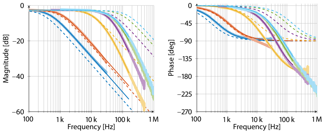
Figure 4.15: Characterization of the PZT4 piezo driver, where dashed lines indicates the white box model, light thick lines the measurement and the thin line the identified behavior. Different low pass filter settings of 0.3 kHz (—), 1 kHz (—), 10 kHz (—), 50 kHz (—), 100 kHz (—) and 150 kHz (—) has been successfully identified.
