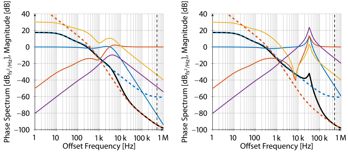
Figure 4.33: GOF for the first design, with (left) and without (right) weight on the controller action, including S (—), T (—), SG (—) and KS (—).
