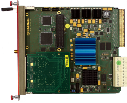
Figure A.4: FMC25 Computation AMC
