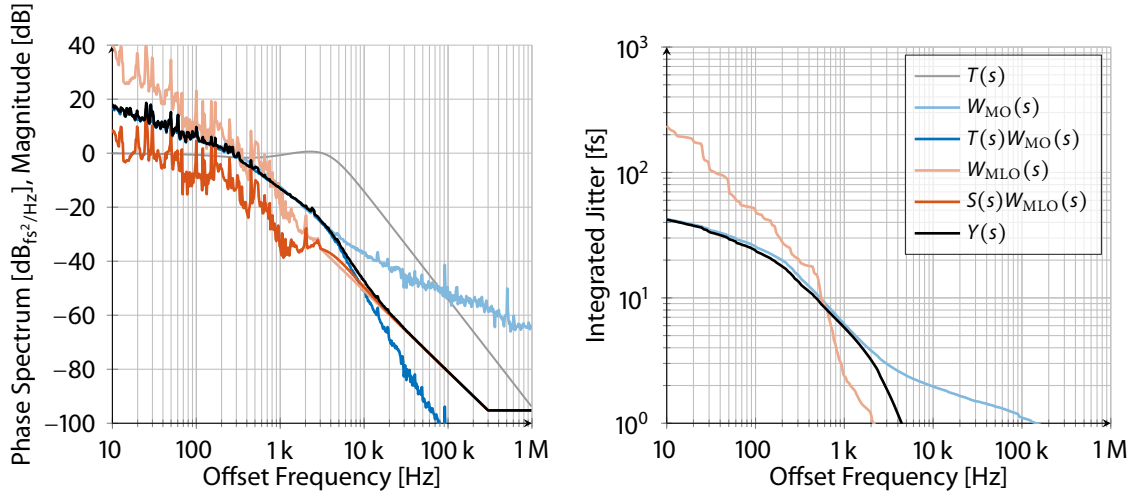
Figure 4.36: Phase noise and integrated timing jitter for the second design.
