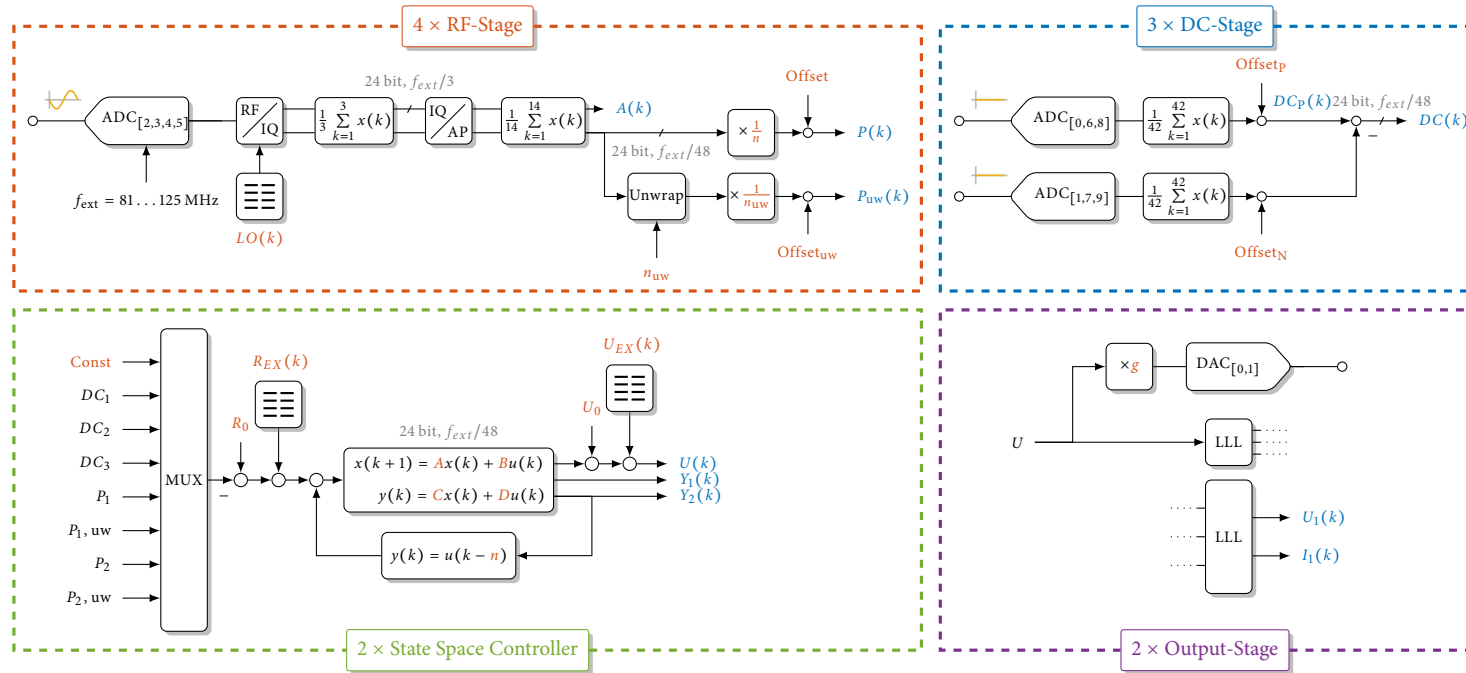
Figure B.1: Simplified block diagram of the MLO firmware.
