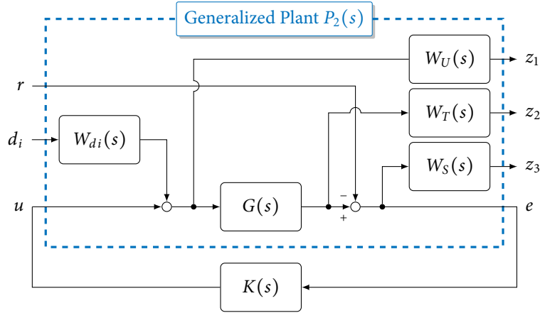
Figure 4.34: Generalized Plant for the second design.
