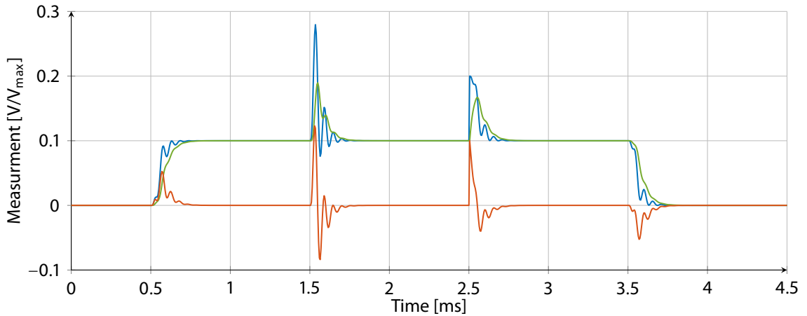
Figure 6.3: Simulation of the timing error after the BAM (—) end-station, the L2RF (—) end-station and the difference between both (—) if the associated LSU is excited by the test sequence.
