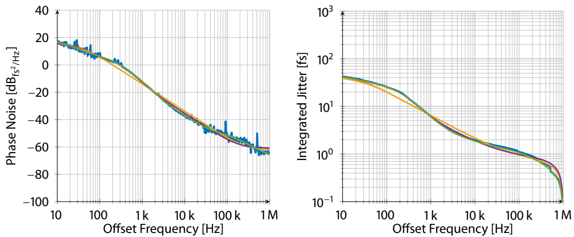
Figure 4.23: Approximation of the MO phase noise (—) with a first (—), second (—), third (—) and fourth (—) order filter.
