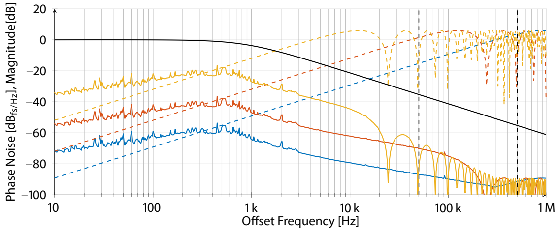
Figure 5.24: MLO phase noise measurable as a disturbance at the link with the short (—), the FLASH (—), and the longest XFEL (—) fiber, the relevant transfer fiber functions (---), and the complementary sensitivity function of the MLO loop (—).
