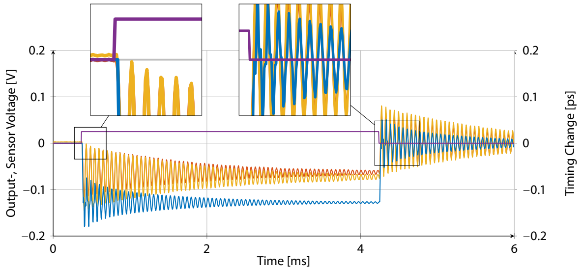
Figure 5.12: Step response of the short links setup G_{\text{Short}}(s) , showing the excitation voltage (—), the sensor measurement in [\frac{V}{V_{\text{max}}}] (—) and in [ps] (—), and the white box model response (—) in [ps].
