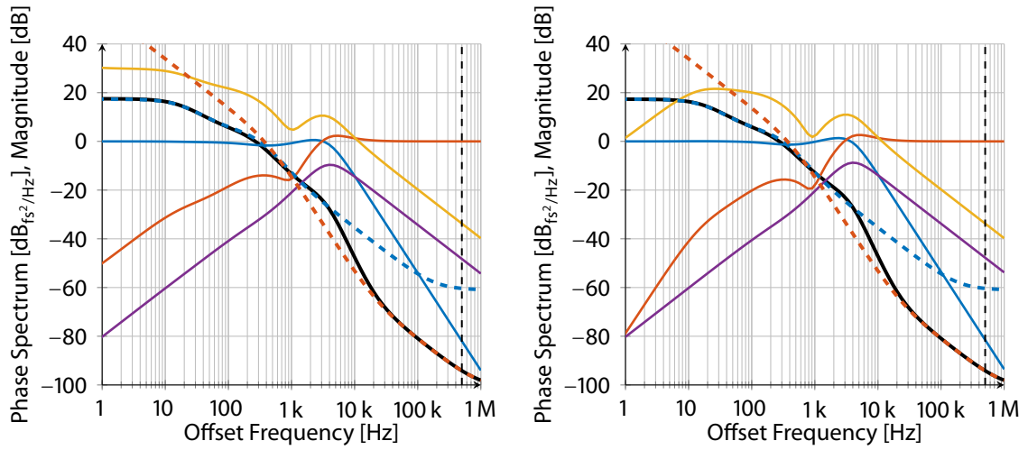
Figure 4.35: GOF of the first (left) and second design (right), with S (—), T (—), SG (—) and KS (—).
