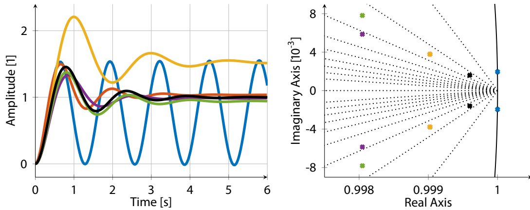
Figure 3.13: Step response (left) and pole location (right) for the example system with 9 fractional bits, sampling frequencies of 2.5 kHz (—), 1.25 kHz (—), 0.833 kHz (—), 0.625 kHz (—), 0.5 kHz (—) and simulated in continuous time (—)
