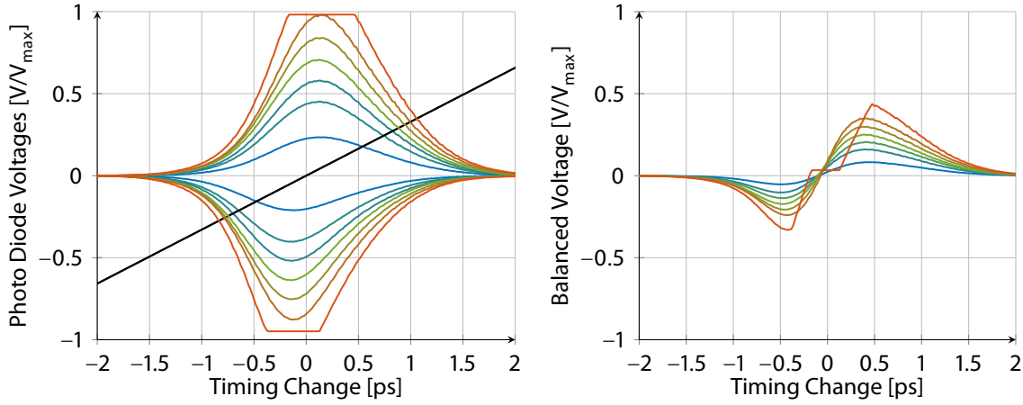
Figure 5.20: Measurement of f_{\text{OXC}} with different LDD currents, of 250 mA (—), 300 mA (—), 325 mA (—), 350 mA (—), 375 mA (—), 400 mA (—), and 450 mA (—). The applied normalized piezo voltage during the sweep is given in (—).
