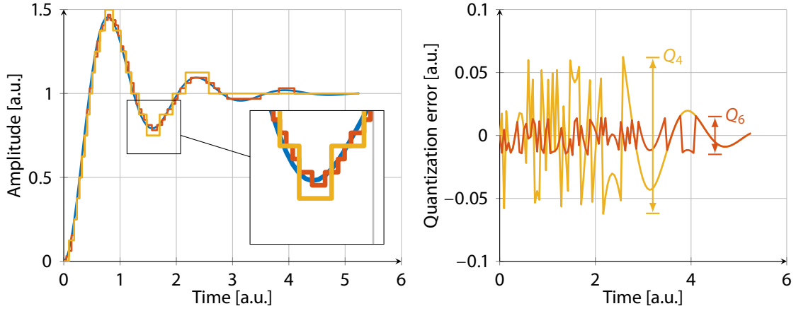
Figure 3.10: Step response (left) and quantization error (right) of this response with 6 (—) and 4 (—) bit compared to the continuous signal (—)
