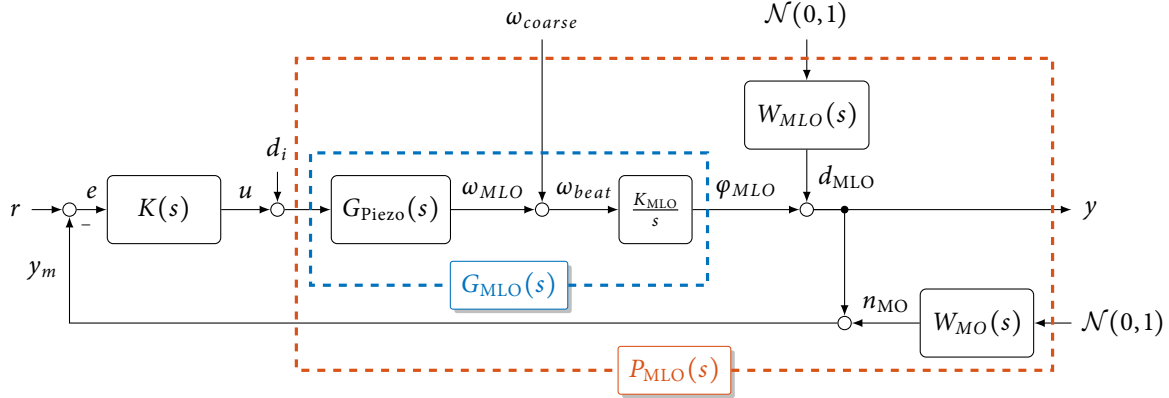
Figure 4.22: Control loop for the MLO system with additional coloring filter.
