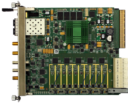
Figure A.1: SIS8300L2 Computation AMC
