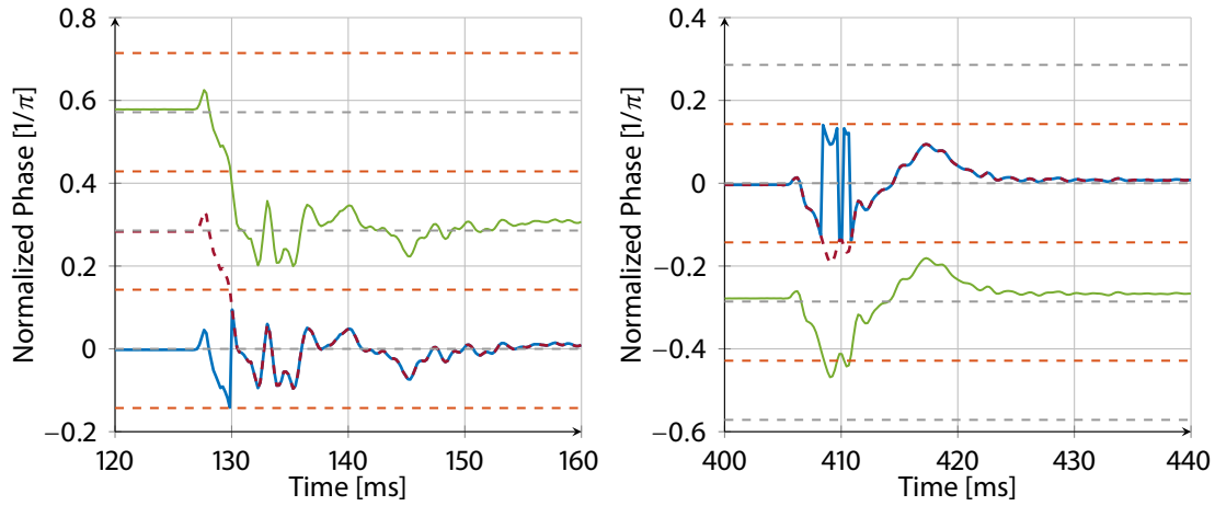
Figure 4.39: Disturbance rejection if locking to the 1516 MHz phase (—) or to the unwrapped phase (---), with the 216 MHz phase (—), the buckets (---) and the stable equilibrium inside the bucket (---).
