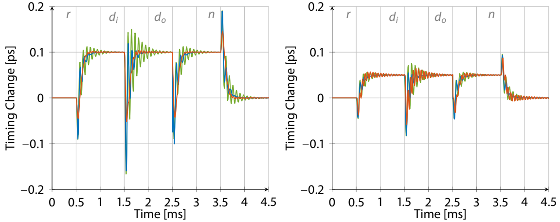
Figure 5.48: Simulation of the PI controller without internal time delay and with a short (—) a 412 m (—) and a 2.542 km (—) long fiber.
