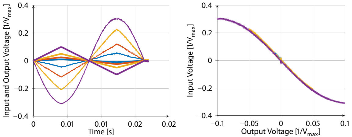
Figure 5.29: Time response (left) and measurement change to input voltage behavior (right) for excitations with an amplitude of 1% (—), 2.5% (—), 5% (—), and 10% (—) close to the working point.
