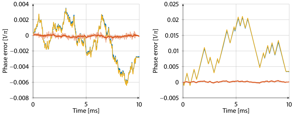
Figure 4.19: Time domain response for the BLWN excitation and the PRB signal with the measurement (—), the simulate response (—), the error of the non-delayed model (—) and the error of the delayed model (—).
