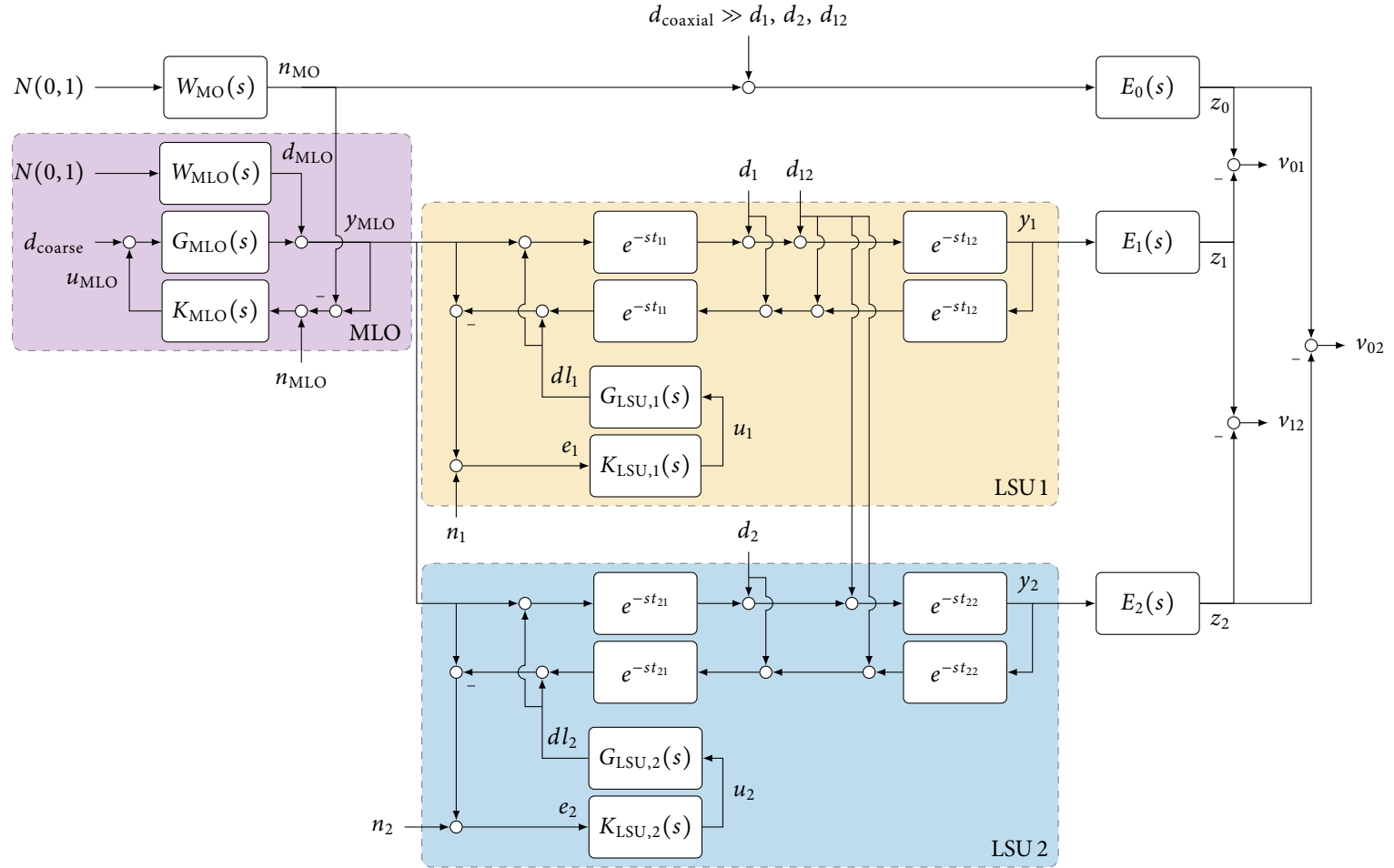
Figure 6.2: Block diagram of the LbSync system with MO, MLO subsystem, two LSU with the end stations E_1(s) and E_2(s) . All signals are expressed in phases w.r.t. the ideal phase of the absolute 216.67 MHz reference signal.
