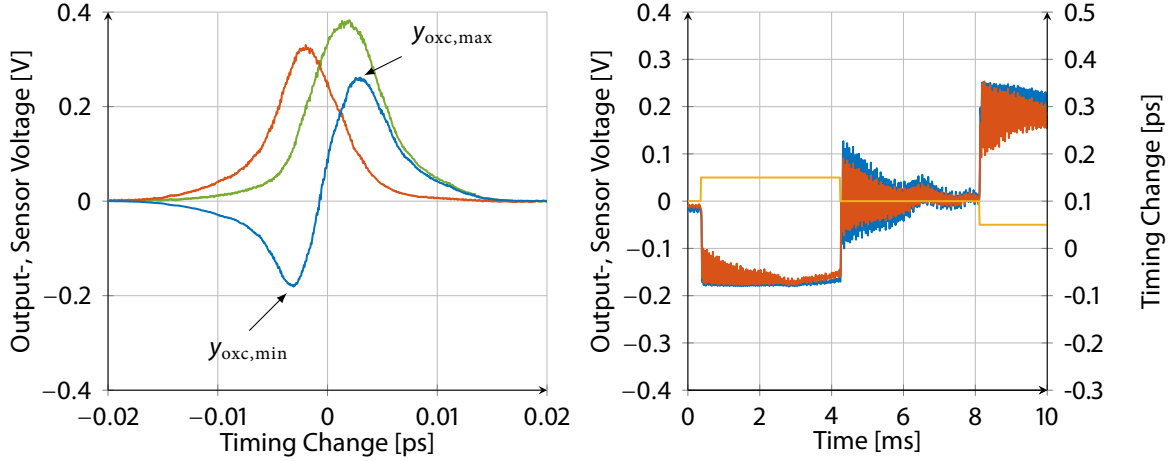
Figure 5.19: Typical measurement of f_{\text{OXC}} (left) with the positive (—), negative (—), and the difference (—) of the correlation pulses, and a step response leaving the linear region (right) with the additional excitation (—).
