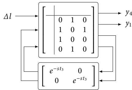
Figure 5.18: LFT model of the fiber link
