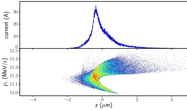
FIG. 6. The longitudinal phase space (LPS) and corresponding current profile is illustrated for the operational point yielding the largest beam brightness, B_{6D} = 1.3 \times 10^{22} , for (\phi, E_0) = (-41.2 \text{ deg}, 123.75 \text{ MV/m}) . The maximum peak current of the bunch is \sim 35 \text{ A} .
