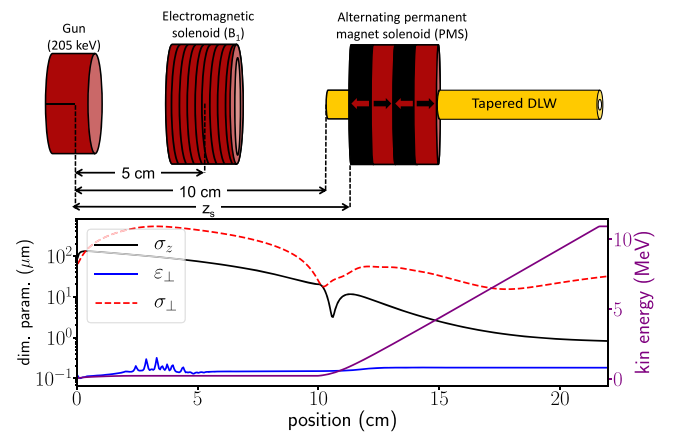
FIG. 1. Diagram of the accelerator concept (top) and corresponding evolution of the bunch's transverse emittance ( \epsilon_r ), rms transverse beam size ( \sigma_r ), longitudinal bunch length ( \sigma_z ) (all left axis) and the kinetic energy (right axis) along the accelerator beamline (bottom). The example corresponds to an operating point (\phi, E_0) = (79.3 \text{ deg}, 106.875 \text{ MV/m}) ; see text for details.
