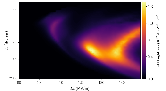
FIG. 5. The final beam brightness B_{6D} = \frac{Q}{\epsilon_x \epsilon_y \epsilon_z} , is illustrated over (\phi, E_0) . The maxima correspond very closely with minimum bunch lengths but differentiations arise from charge losses and, e.g., beam dilution.
