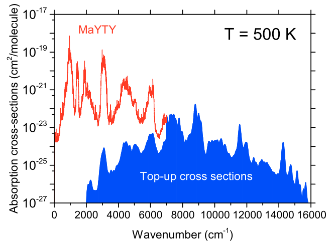
Figure 11. The vibrational ‘top-up’ cross-sections of \text{C}_2\text{H}_4 computed using the vibrational line list with the three-band model at T = 500 \text{ K} (dark blue area) and the ro-vibrational intensities generated using the ExoMol line list with the Gaussian line profile of HWHM = 1 \text{ cm}^{-1} (red line).
