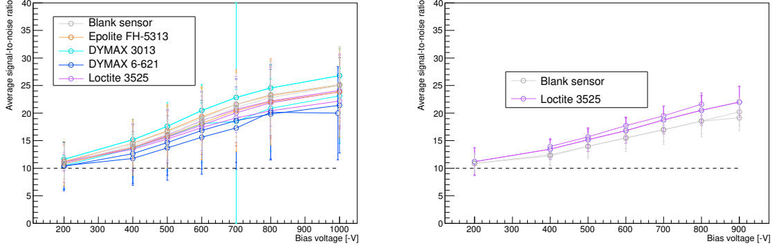
(a) SNR for sensors irradiated with 23 MeV protons at KIT (b) SNR for sensors irradiated with reactor protons at JSI
