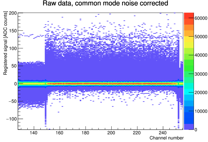
Figure 6.16: ALiBaVa raw data for 500,000 events after base value subtraction and common mode noise correction. The width of the background distribution, i.e. the distribution around readout signal = 0 ADC, has been decreased with respect to the signal before common mode noise correction.
