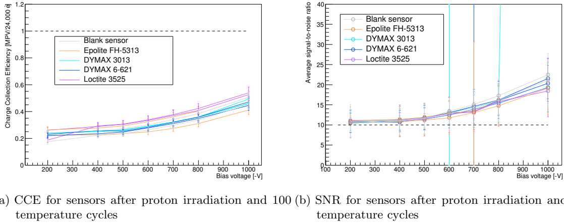
Figure 6.38: CCE and SNR for ATLAS07 sensors (FZ1, narrow strip pitch) with and without glue after proton irradiation and temperature cycling. CCE and SNR are comparable within uncertainties for sensors with and without glue.
