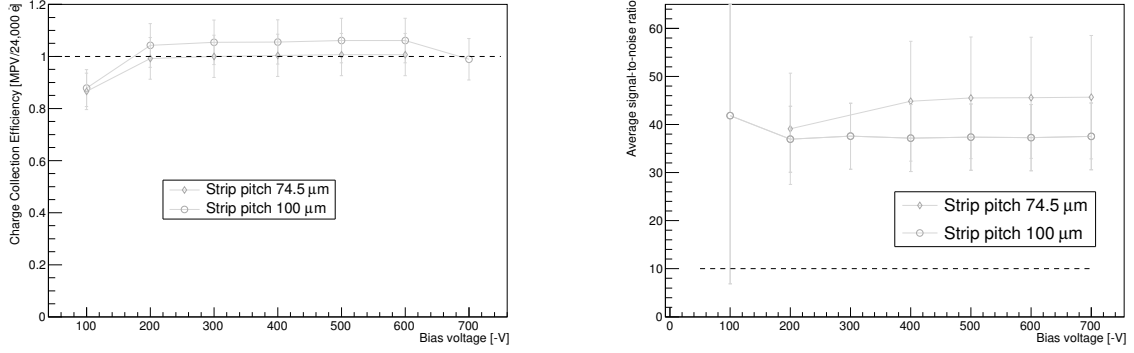
(a) Charge collection efficiency (CCE) of two blank ATLAS07 miniature sensors: both sensors have a CCE agreeing with 100 % within uncertainties. (b) Signal-to-noise ratios of two blank ATLAS07 miniature sensors: due to a higher noise, the BZ6 sensor has a lower SNR despite showing a larger CCE.
