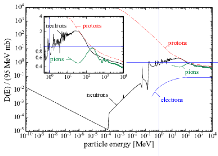
Figure 3.5: Displacement damages for different particles relative to the neutron equivalent fluence \Phi_{eq} [54]
