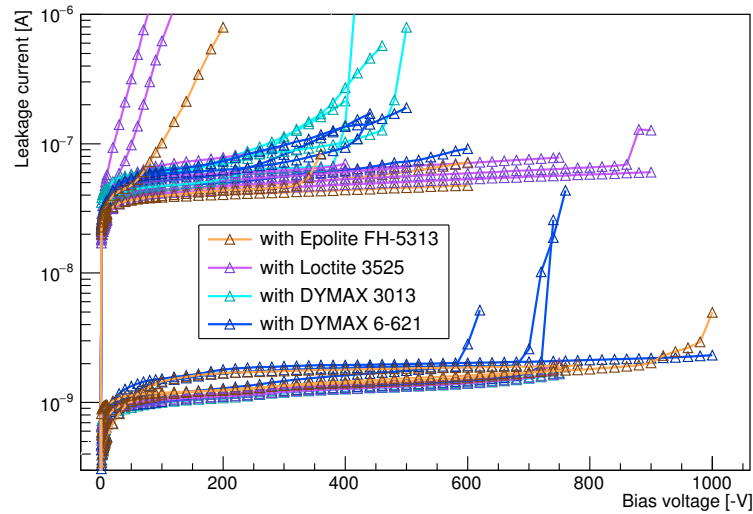
(b) Leakage currents of sensors with glue
