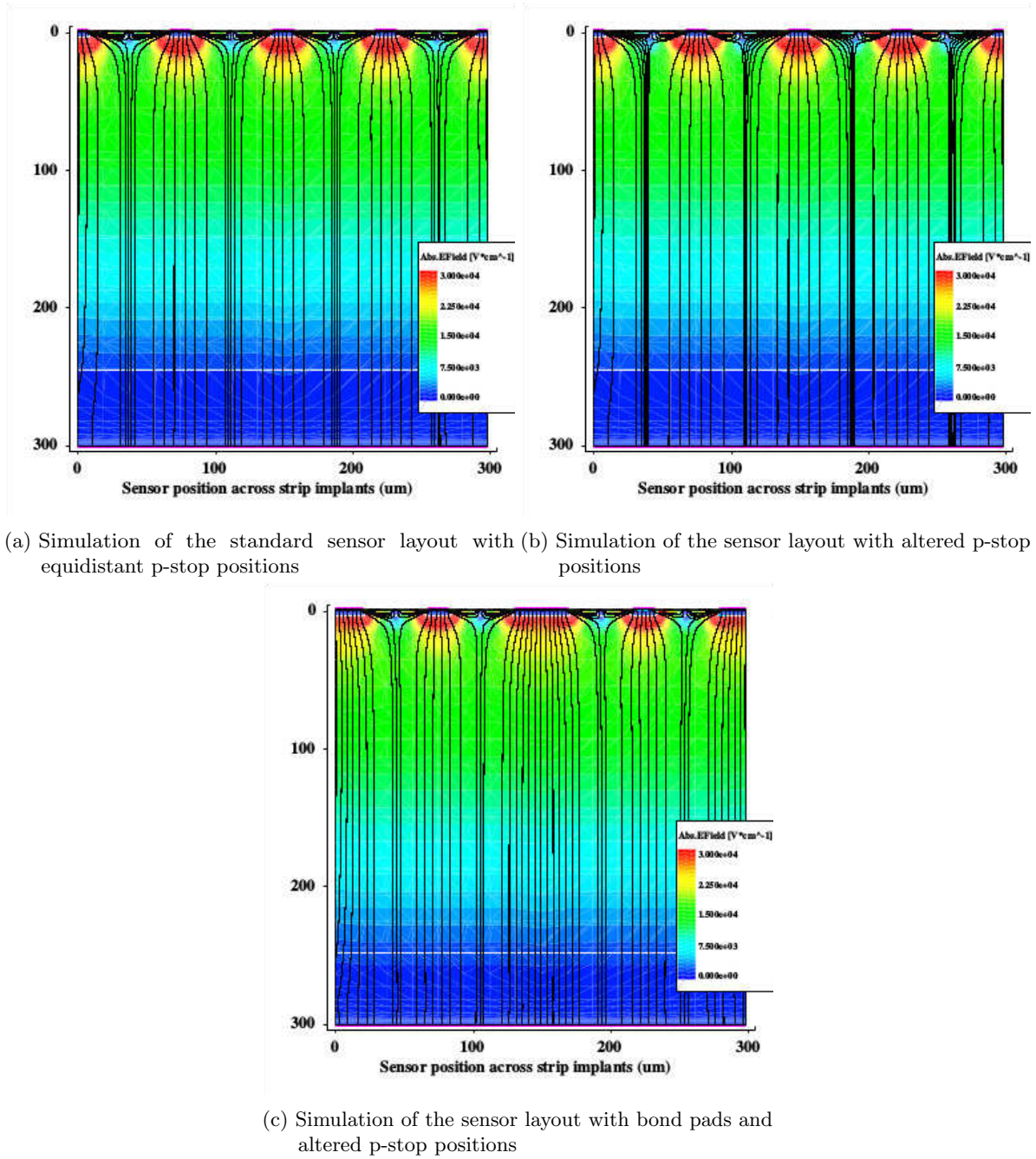
Figure 9.15: 2D TCAD simulation of the electric field and its streamlines of a silicon strip sensor. The simulated cross-section of the sensor shows a width and thickness of 300\text{ }\mu\text{m} . A reverse bias of -300\text{ V} is applied at the back side of the sensor at 300\text{ }\mu\text{m} . The simulations are done for a resistivity of 2.5\text{ k}\Omega\text{-cm} , to study the effect of different widths of the metal contact and strip implant, and the effect of different p-stop positions. Figures from [143].
