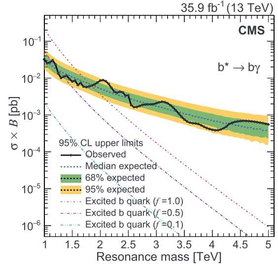
Fig. 5. The observed and expected upper limits at 95% CL on \sigma \mathcal{B} as a function of the mass of the excited b quark, for f = 1.0 . The limits are compared with theoretical predictions for excited b quark production for three couplings. The inner (green) band and the outer (yellow) band indicate the regions containing 68 and 95%, respectively, of the mean limits under the background-only hypothesis.
