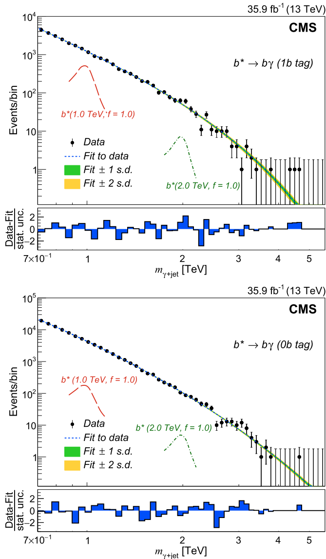
Fig. 3. The \gamma + bjet invariant mass distribution in data (black points) used for the b^* analysis, after final selection for (upper) 1b tag category and (lower) 0b tag category. The result of the fit to the data using the parametrization defined in Eq. (2) is shown by the blue dashed curve with associated bands indicating the uncertainty. The bin-by-bin pull, (\text{Data-Fit})/(\text{stat. unc.}) , where the denominator refers to the statistical uncertainty in data, is also presented. The green and yellow bands correspond to 1 and 2 standard deviations, respectively from the mean value. Simulations of excited b quark signals representing the expected excess of signal events over the background are shown for the 1b and 0b tag categories for the mass values of 1.0 and 2.0 TeV for f = 1.0 .
