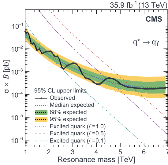
Fig. 4. The observed and expected upper limits at 95% CL on \sigma \mathcal{B} as a function of the mass of the excited quark, for f = 1.0 . The limits are compared with theoretical predictions for excited quark production for three couplings. The inner (green) band and the outer (yellow) band indicate the regions containing 68 and 95%, respectively, of the mean limits under the background-only hypothesis.
