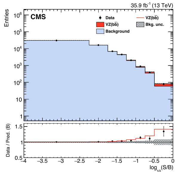
Fig. 8. Combination of all channels in the VZ search, with Z \rightarrow b\bar{b} into a single event BDT distribution. Events are sorted in bins of similar expected signal-to-background ratio, as given by the value of the output of their corresponding BDT discriminant. The bottom inset shows the ratio of the data to the predicted background, with a red line overlaying the expected SM contribution from VZ with Z \rightarrow b\bar{b} .
