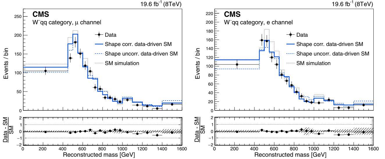
FIG. 3. The reconstructed VLQ candidate mass in the W^-qq category for the muon channel (left) and the electron channel (right), for the background prediction and the data. The solid bold (blue) line is the background distribution estimated from data, with a final shape correction that accounts for the difference between the W + \text{jets} simulation in the control region and the W^-qq signal region. The dashed (blue) line is the same, but without the shape correction. The dotted (grey) line represents the SM prediction from simulation. The lower panel shows the ratio of the data to the data-driven background distribution with shape corrections. For bins from 1000 GeV onwards, a wider bin width is chosen to reduce statistical uncertainties in the background estimation from the data control region. The horizontal error bars on the data points indicate the bin width.
