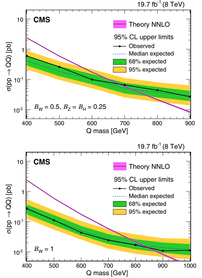
FIG. 17. The 95% C.L. exclusion limits on the production cross section determined assuming different sets of model parameters ( \mathcal{B}_W = 0.5, \mathcal{B}_Z = 0.25 (upper), and \mathcal{B}_W = 1 (lower)) as a function of the hypothetical VLQ mass, and for the scenario where only strong pair production of the VLQs is considered. The median expected and observed exclusion limits are indicated with a dashed and a solid line, respectively. The inner (green) band and the outer (yellow) band indicate the regions containing 68% and 95%, respectively, of the distribution of limits expected under the background-only hypothesis. The cross section from a full NNLO calculation [25], including uncertainties in the PDF description and the renormalization and factorization scales, is shown by the magenta band.
