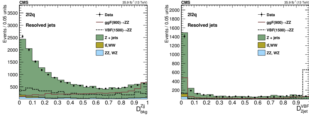
Figure 5: Distributions of the D_{bkg}^{Zij} (left) and D_{jet}^{VBF} (right) discriminants in the signal region for the resolved selection. The points represent the data, the stacked histograms the expected background from simulation, and the open histograms the expected signal.
