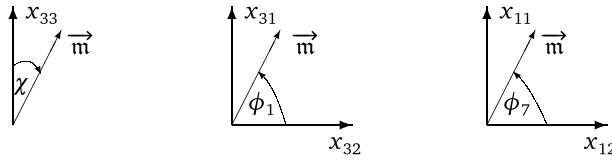
Fig. 1. Visualisation of the angles \chi , \phi_1 , and \phi_7 . The other \phi_i follow analogously; the coordinate x_{ij} represents the axis relating i -th and j -th generation \sim \psi_{L,i} \psi_{R,j} .
