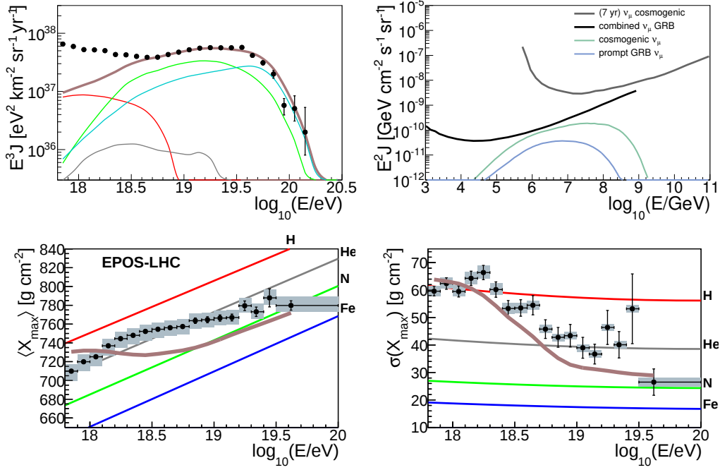
Figure 4: Figure taken from [3] – Cosmic-ray and neutrino observables obtained with the best-fit parameters in the Mixed Composition Ankle Model. Upper left: simulated energy spectrum of UHECR (multiplied by E^3 ) compared to data from [19]. Spectra at Earth are grouped according to the mass number as follows: A = 1 (red), 2 \leq A \leq 4 (grey), 5 \leq A \leq 22 (green), 23 \leq A \leq 28 (cyan), total (brown). Upper right: Prompt and cosmogenic (muon flavor) neutrino spectra. The differential limits are defined as in [6]. Bottom: average and standard deviation of the X_{\text{max}} distribution as predicted (assuming EPOS-LHC [23] for UHECR-air interactions) for the model versus pure ( 1 H (red), 4 He (grey), 14 N (green) and 56 Fe (blue)) compositions, compared to data from [24].
