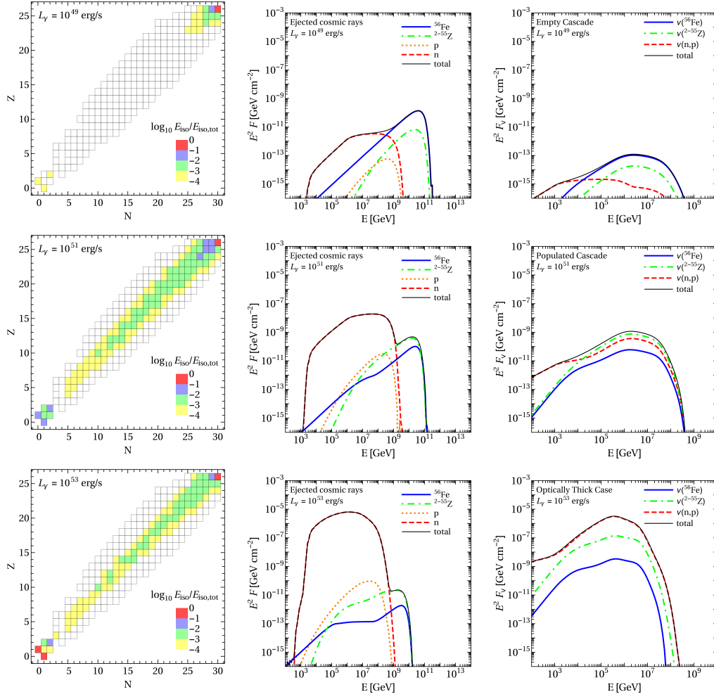
Figure 1: Figure taken from [3] – Nuclear cascade (left), ejected cosmic ray fluence per shell (center) and neutrino fluence per shell (right) as a function of the energy in the observer’s frame, for the injection of pure ^{56}\text{Fe} . First row: Example for the “Empty Cascade” source class (isotropic luminosity L_\gamma = 10^{49} \text{ erg s}^{-1} ). Second row: Example for the “Populated Cascade” source class ( L_\gamma = 10^{51} \text{ erg s}^{-1} ). Third row: Example for the “Optically Thick Case” (to nucleons and nuclei) source class ( L_\gamma = 10^{53} \text{ erg s}^{-1} ). The different curves in the central panels correspond to the different isotopes, according to legend. The different curves in the right panels show the contribution of the photo-meson production off the primary ( ^{56}\text{Fe} ) and secondary isotopes produced in the photo-disintegration, where the proton/neutron contribution is separated. The other GRB parameters are: R \simeq 10^{8.3} \text{ km} , \Gamma = 300 , \xi_{\text{Fe}} = 10 , \epsilon'_{\gamma, \text{br}} = 1 \text{ keV} and z = 2 .
