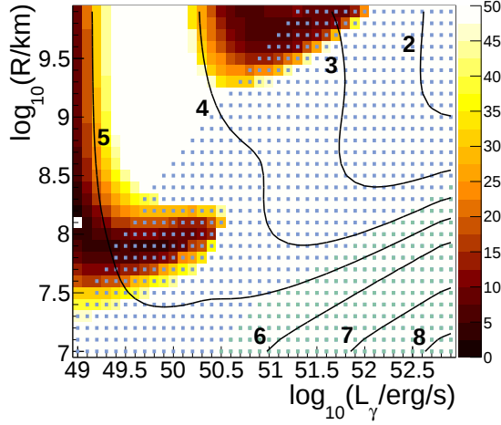
Figure 3: Figure taken from [3] – Parameter space scan for Mixed Composition Ankle Model in the internal shock scenario. Here \sqrt{\chi^2 - \chi_{\min}^2} is shown as a function of R and L_\gamma for the fit to cosmic-ray data of the Pierre Auger Observatory [19, 4] above 10^{19} eV, including a penalty for the overshooting of the flux at lower energies. The blue squares mark the current (90% C.L.) IceCube-excluded region from the GRB stacking analysis from Northern and Southern sky muon tracks [20, 21], while the green ones mark the current (90% C.L.) IceCube-excluded region from the cosmogenic neutrino analysis [22], applied to \nu_\mu + \bar{\nu}_\mu . The contours show the nuclear loading ( \log_{10} \xi ).
