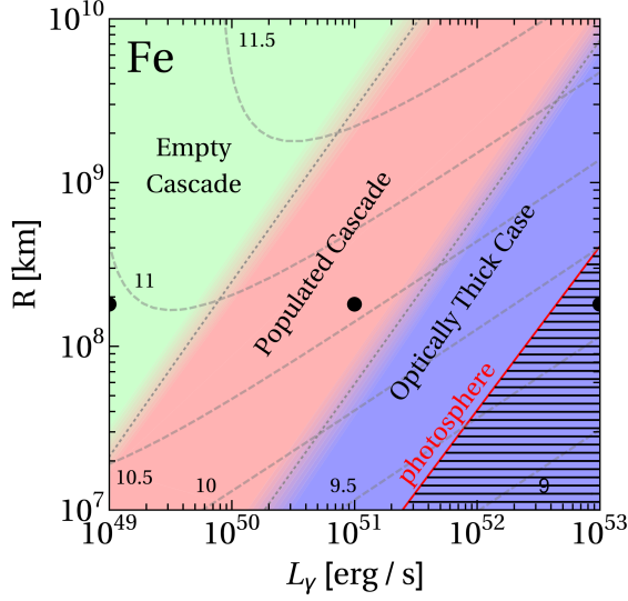
Figure 2: Figure taken from [3] – Nuclear cascade class as a function of luminosity L_\gamma and collision radius R in the internal shock scenario, for pure ^{56}\text{Fe} at injection. The other parameters are the same as in Fig. 1. Black dots indicate the position of the examples shown in Fig. 1. The gray dashed contours display \log_{10}(E_{i,\text{max}}[\text{GeV}]) in the observer’s frame. Note that in this figure we scale t_v \propto R .
