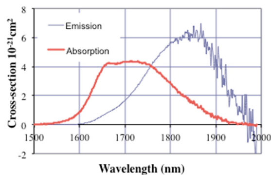
Figure 4. Absorption and emission cross section of the 1.0% \text{Tm}_2\text{O}_3 -doped TeNbKTm samples deduced by using the McCumber analysis.
