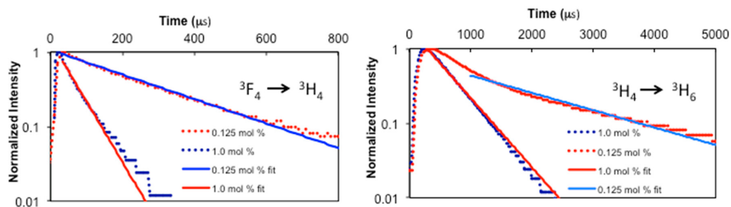
Figure 2. Measured fluorescence decay curves and the exponential fits of the (a) ^3\text{F}_4 level and (b) ^3\text{H}_4 level for the two \text{Tm}_2\text{O}_3 : \text{TeO}_2 - \text{K}_2\text{O} - \text{Nb}_2\text{O}_5 (TeNbKTm) samples with \text{Tm}_2\text{O}_3 concentrations of 1.0 and 0.125 mol % [29].
