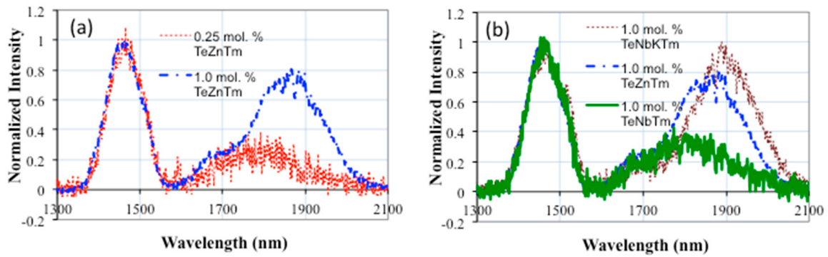
Figure 3. (a) Emission spectra of the two transitions of the \text{Tm}^{3+} ion originating from ^3\text{F}_4 and ^3\text{H}_4 levels to the ground level for the glass host TeZnTm with \text{Tm}_2\text{O}_3 concentrations of 1.0 and 0.25 mol %; (b) Emission spectra of the three glass hosts TeNbKTm, TeZnTm and TeNbTm, each with 1.0 mol % \text{Tm}_2\text{O}_3 doping.
