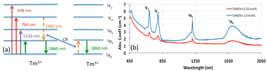
Figure 1. (a) Energy level diagram of the \text{Tm}^{3+} ion. CR: Cross-relaxation (b) Absorption spectra of two \text{Tm}_2\text{O}_3 : \text{TeO}_2 - \text{Nb}_2\text{O}_5 glass samples with \text{Tm}_2\text{O}_3 concentrations of 1.0 and 0.25 mol % in the range of 450–2050 nm. The corresponding absorption bands from the ground state ( ^3\text{H}_6 ) are indicated.
