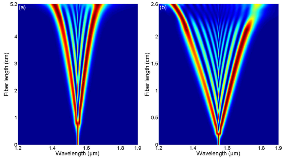
Fig. 3. Spectral evolution for different combinations of fiber length and input pulse energy: (a) 95-nJ pulse, fiber length up to 5.2 cm and (b) 380-nJ pulse, fiber length up to 2.6 cm. For both cases, the input pulse is a hyperbolic-secant pulse with 300-fs duration centered at 1.55 \mu\text{m} . The fiber has 10- \mu\text{m} MFD, -10 \text{ fs}^2/\text{mm} GVD, and 100 \text{ fs}^3/\text{mm} TOD at 1.55 \mu\text{m} .
