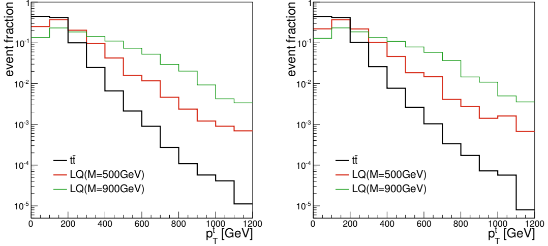
Figure 7.7: Shape comparison of p_T^l for different LQ mass hypotheses and the t\bar{t} background in the \mu + \tau_h + \text{jets} (left) and e + \tau_h + \text{jets} (right) final state.
