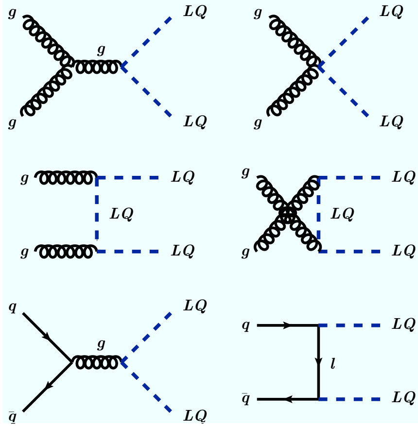
Figure 2.2: Leading-order Feynman diagrams of LQ pair production.
