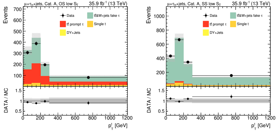
Figure B.6: Distributions of p_T^t in the control region \text{CR}_{\text{test}} . The events are separated into OS (left) and SS (right) regions. In the bottom panel, the dark grey shaded area represents the statistical uncertainties and the light grey shaded area corresponds to the total uncertainties.
