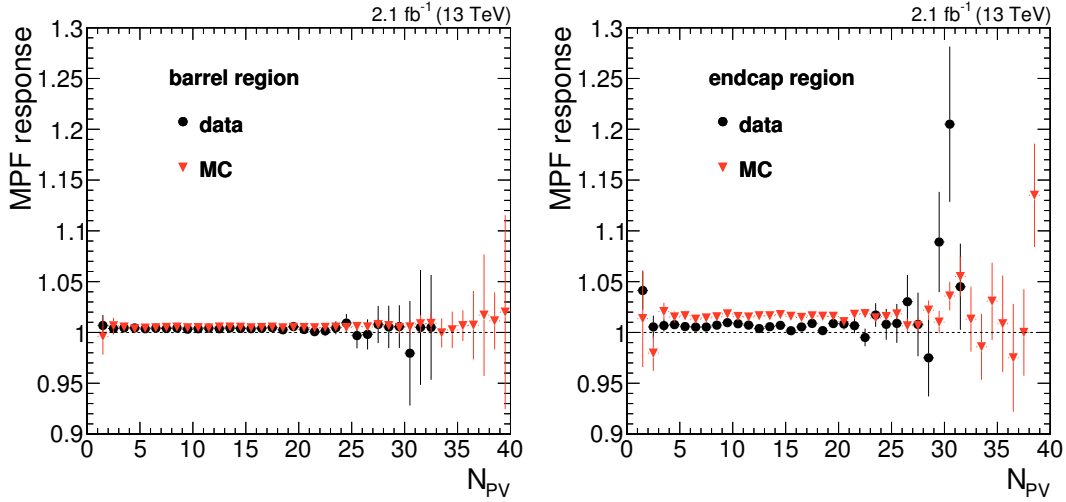
Figure 6.11: Relative response of data and simulation as a function of the number of primary vertices for one bin in the in the barrel (left) and for one bin in the endcap (right) region.
