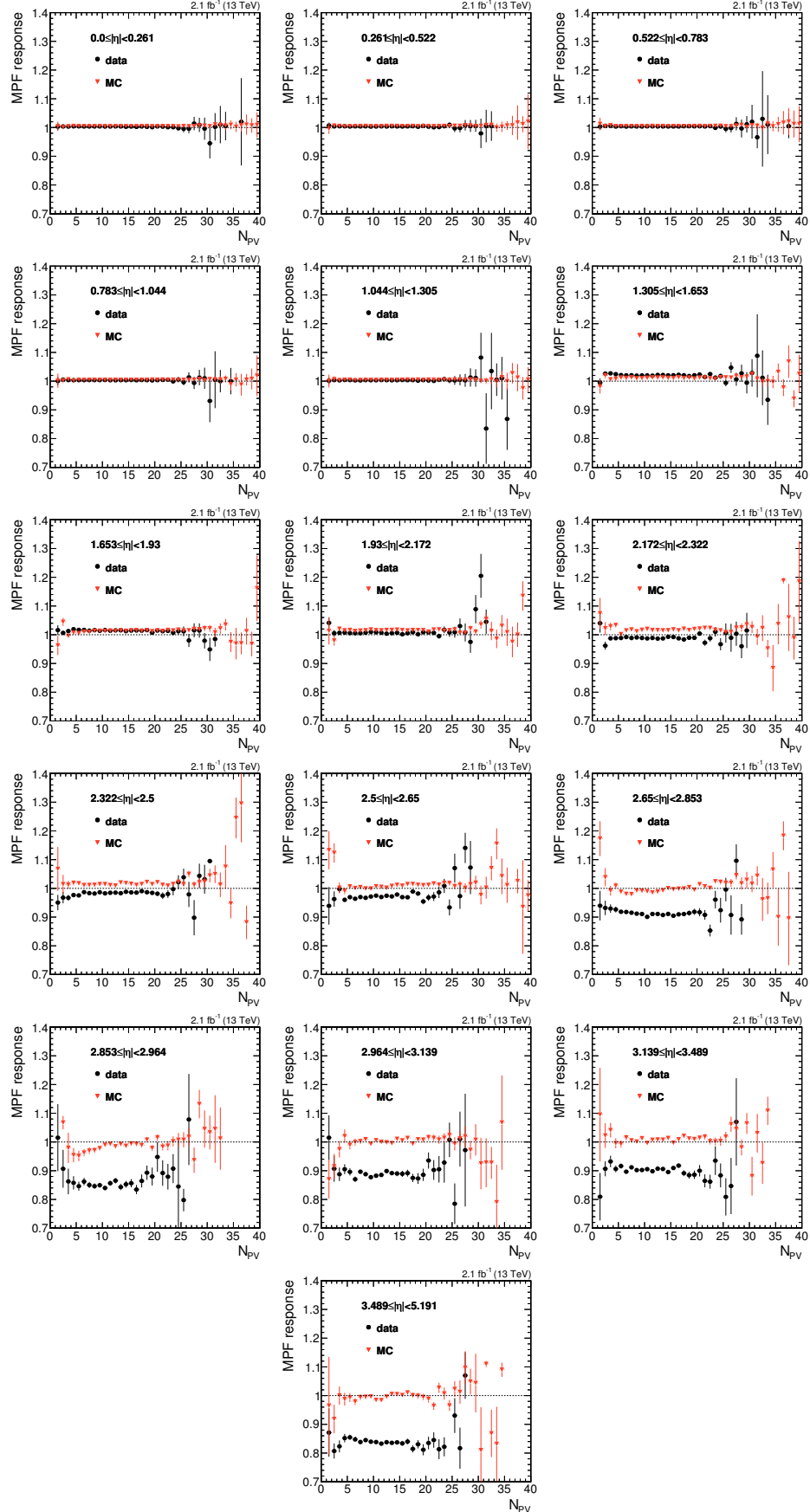
Figure A.5: Relative response as a function of the number of primary vertices for each bin of |\eta| .
