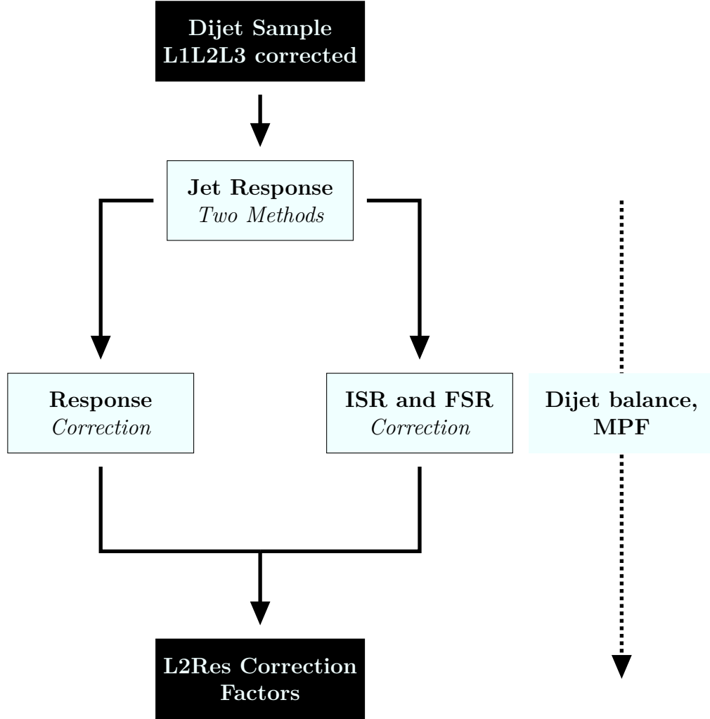
Figure 6.1: Determination of L2Res correction factors. The L1 and the MC truth corrections are applied to a dijet sample. Jet responses are calculated by using the p_T balance and the missing transverse energy projection fraction (MPF) methods. Jet response corrections as well as ISR and FSR corrections are considered to determine the L2Res correction factors.
