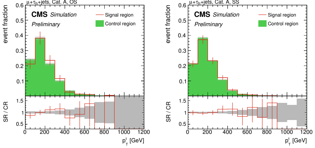
Figure 7.14: Shape comparison between signal region ( SR_A ) and control region ( CR_A ) of the p_T^l distribution after applying the correction factors. The comparison is shown inclusively in S_T after applying the full selection in the \mu + \tau_h + \text{jets} final state in the OS (left) and the SS (right) category. Published in Ref. [1].
