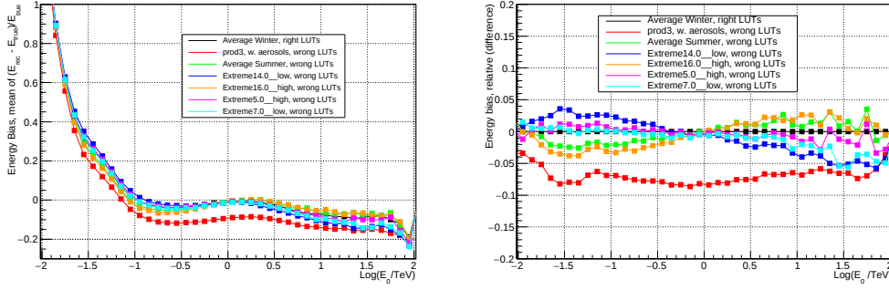
Figure 7: Energy bias (left) for the different molecular profiles and the relative difference compared to Average Winter (see text). The Average Winter LUTs have been used for all atmospheric models.
