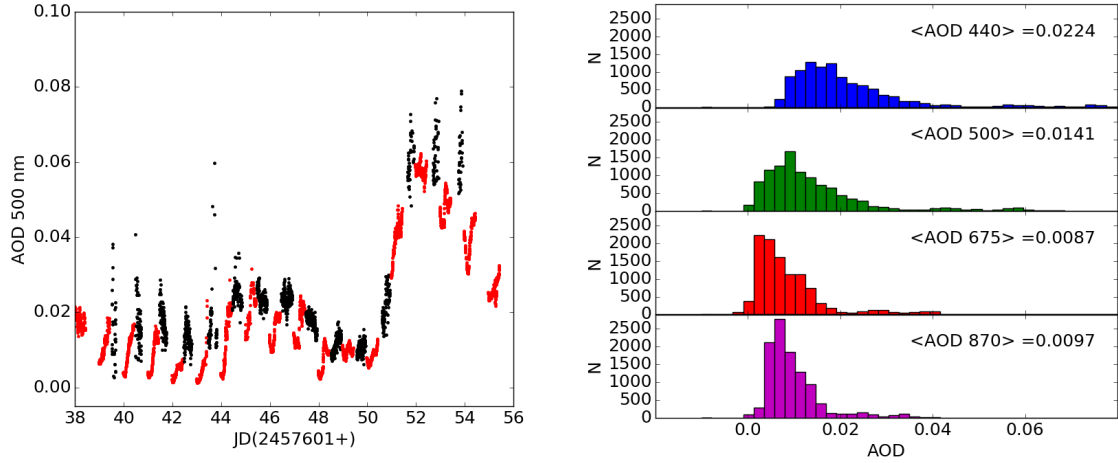
Figure 5: Left: Example of the time dependence of AODs in the 500 nm passband for diurnal (red) and nocturnal (black) measurements combined. Right: overall distribution of AODs in four photometric passbands.
