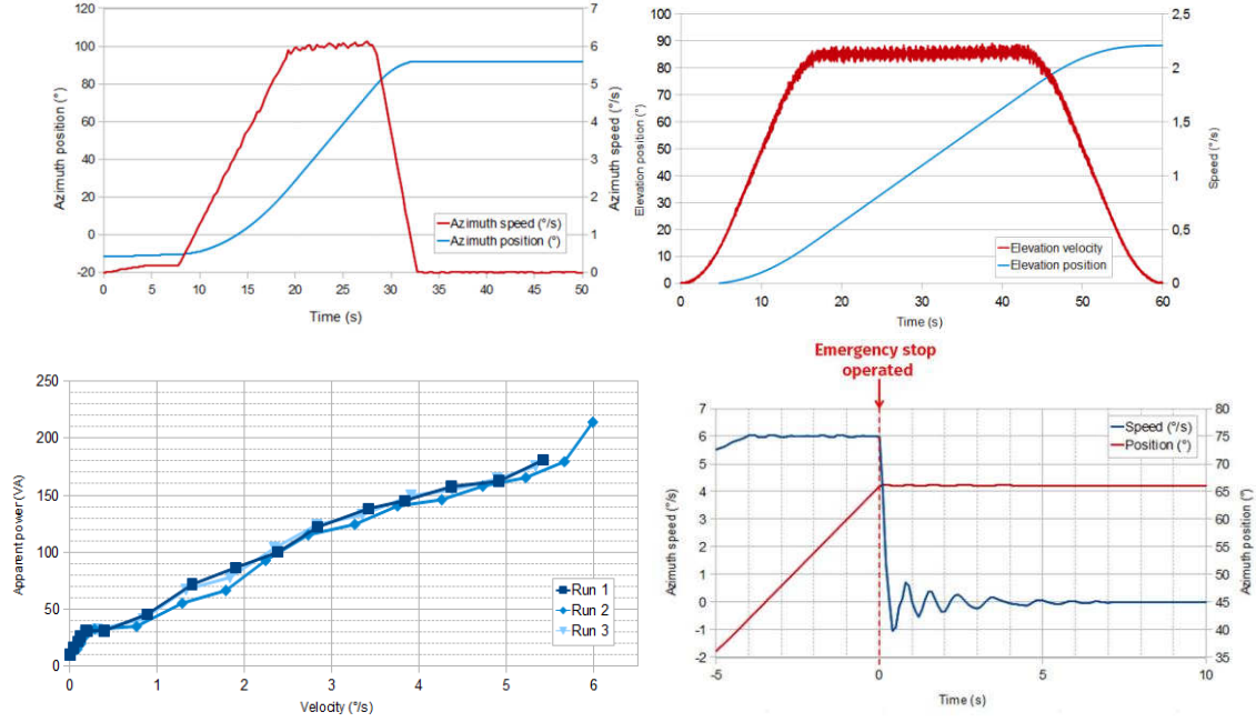
Figure 3: Mechanical and drives performances. Upper panel: azimuth and elevation positions (°) and velocities (°/s). Lower panel: apparent power (VA) versus velocity (°/s) of the azimuth axis, at 20^\circ in elevation (left), and test of emergency stop (right).
