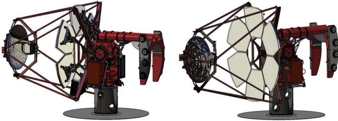
Figure 6: GCT final design proposed for the SST sub-array of CTA
