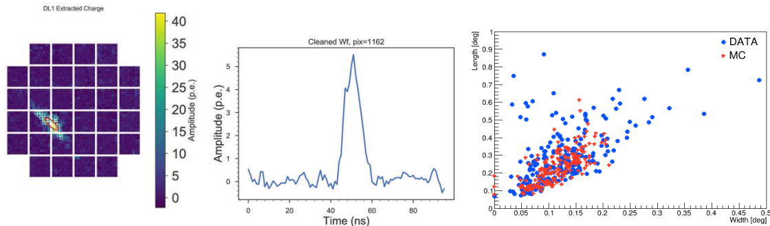
Figure 5: (a) Left panel – Camera image of one Cherenkov event and waveform of the brightest pixel in that image, showing its time evolution over nanoseconds (middle). (b) Right panel - Comparing Cherenkov data and Monte Carlo simulations: Distribution of the cosmic showers registered during one observing run in Meudon (March 30th, 2017) in the plane “length-width” of their images (blue dots) and of the showers generated for the same setup using CORSIKA and sim_telarray simulation tools (red crosses).
