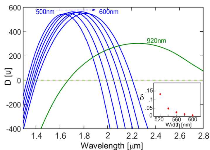
Fig. 6. Dispersion of waveguide varying in width from 500 nm to 600 nm (in blue) shown along with W1 (green) for comparison. The inset shows \delta for waveguides at 1.94 \mu\text{m} . Unit of D is ps 2 /nm 2 /km.
