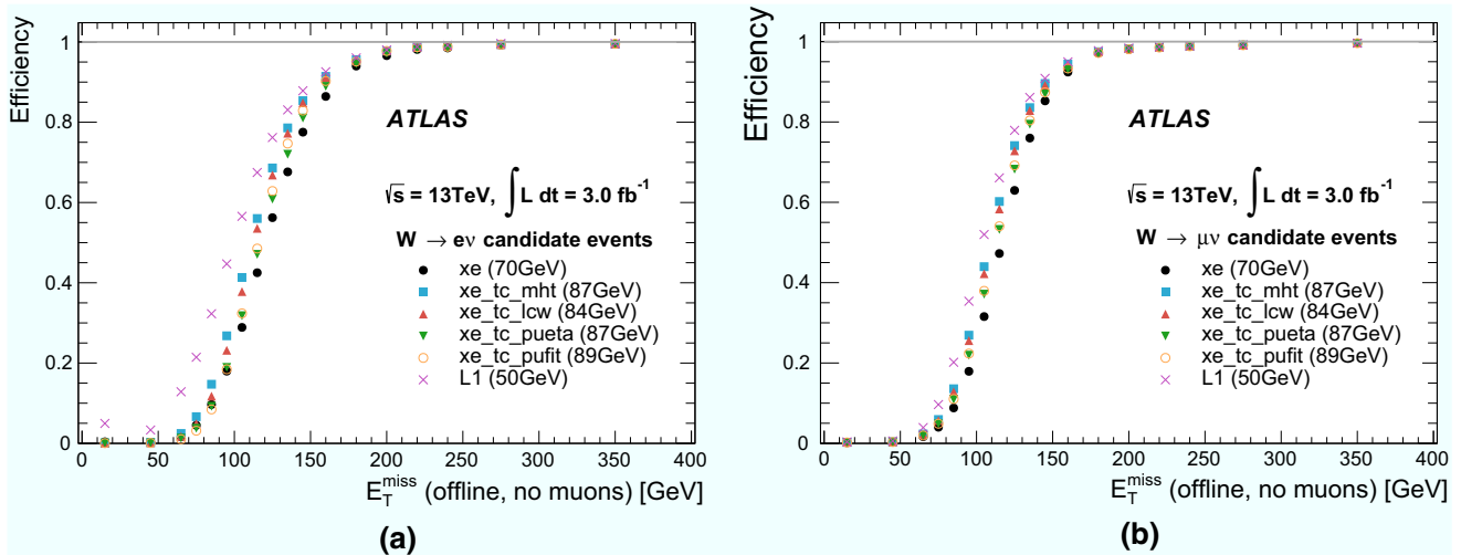
Fig. 41 E_T^{\text{miss}} trigger efficiency curves with respect to the E_T^{\text{miss}} reconstructed offline without muon corrections for all events passing the a W \rightarrow e\nu or b W \rightarrow \mu\nu selections. The different efficiencies were mea-
