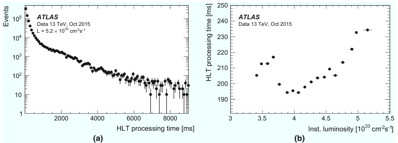
Fig. 8 a HLT processing time distribution per event for an instantaneous luminosity of 5.2 \times 10^{33} \text{ cm}^{-2} \text{ s}^{-1} and average pile-up \langle \mu \rangle = 15 and b mean HLT processing time as a function of the instantaneous luminosity
