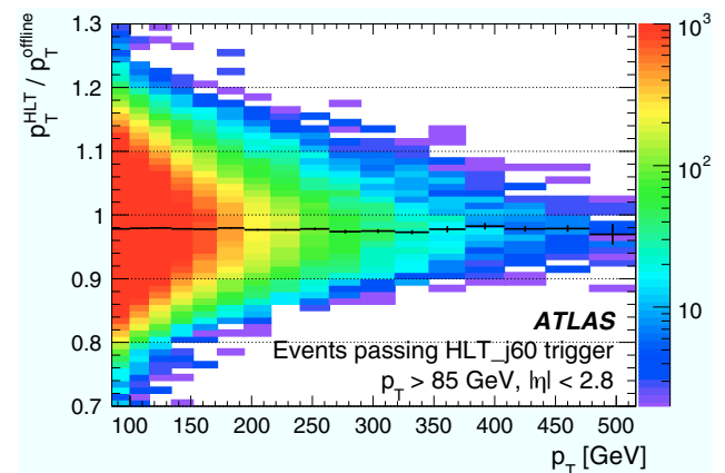
Fig. 32 Comparison between the jet energy scales of trigger and offline jets. The black points represent the mean of the distribution at a given p_T value. The 2% shift is due to differences in the jet calibration applied online and offline
