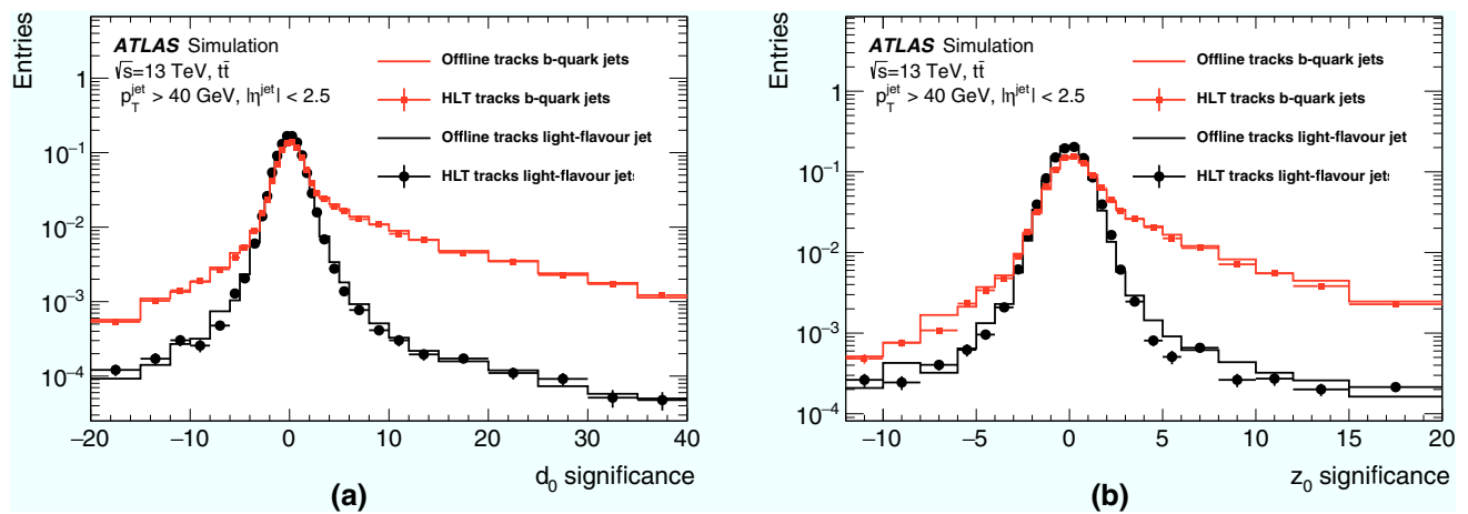
Fig. 44 a Transverse and b longitudinal impact parameter significance for tracks associated with light-flavour (black) and b-quark (red) jets measured in a sample of simulated t\bar{t} events. The solid lines show the distribution for the offline tracks. The points show the corresponding distribution for tracks used in the b-jet trigger. The impact parameter
