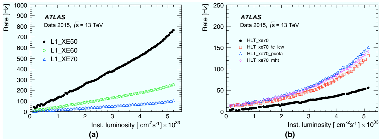
Fig. 40 E_T^{\text{miss}} trigger rates (a) at L1 and (b) for various HLT algorithms operating with nominal thresholds of 70 GeV. The HLT algorithms are each seeded by L1_XE50. Rates are shown as a function of instantaneous
