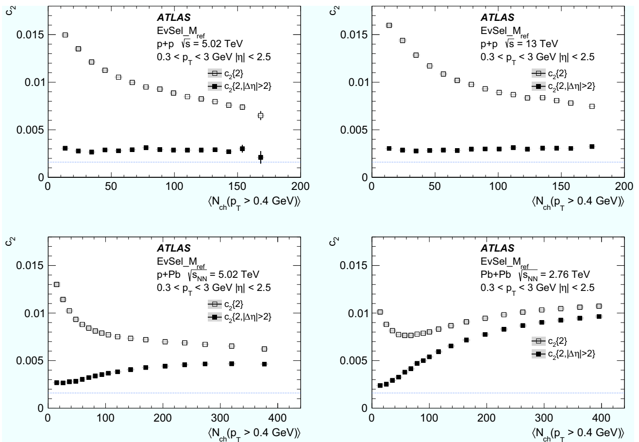
Fig. 4 Comparison of c_2\{2\} (open symbols) and c_2\{2, |\Delta\eta| > 2\} (filled symbols) for reference particles with 0.3 < p_T < 3.0 \text{ GeV} for pp collisions at \sqrt{s} = 5.02 and 13 \text{ TeV} , p + \text{Pb} collisions at \sqrt{s_{NN}} = 5.02 \text{ TeV} and low-multiplicity \text{Pb} + \text{Pb} collisions at \sqrt{s_{NN}} = 2.76 \text{ TeV} . The
