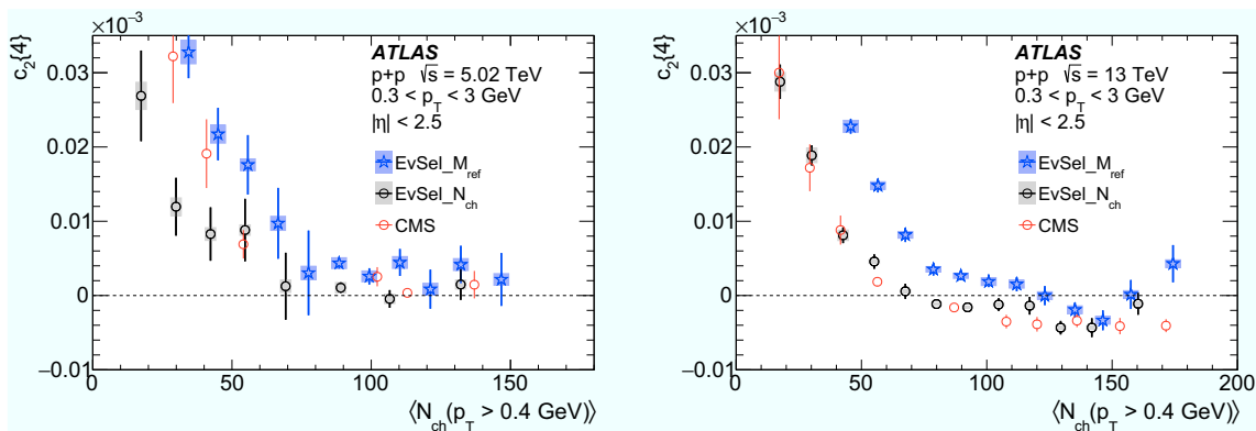
Fig. 14 Comparison of the ATLAS and CMS [45] results for c_2\{4\} cumulants in pp collisions at 5.02 TeV (left) and 13 TeV (right) shown as a function of \langle N_{\text{ch}}(p_T > 0.4 \text{ GeV}) \rangle . The ATLAS results are shown for two event selections: \text{EvSel}_{M_{\text{ref}}} and \text{EvSel}_{N_{\text{ch}}} with the error
