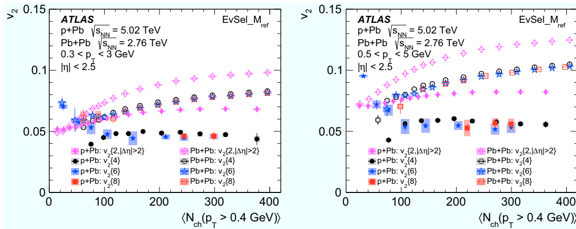
Fig. 10 Comparison of v_2\{2, |\Delta\eta| > 2\} , v_2\{4\} , v_2\{6\} and v_2\{8\} as a function of \langle N_{\text{ch}}(p_T > 0.4 \text{ GeV}) \rangle for p + \text{Pb} collisions at \sqrt{s_{\text{NN}}} = 5.02 \text{ TeV} and low-multiplicity \text{Pb} + \text{Pb} collisions at \sqrt{s_{\text{NN}}} = 2.76 \text{ TeV} . The
