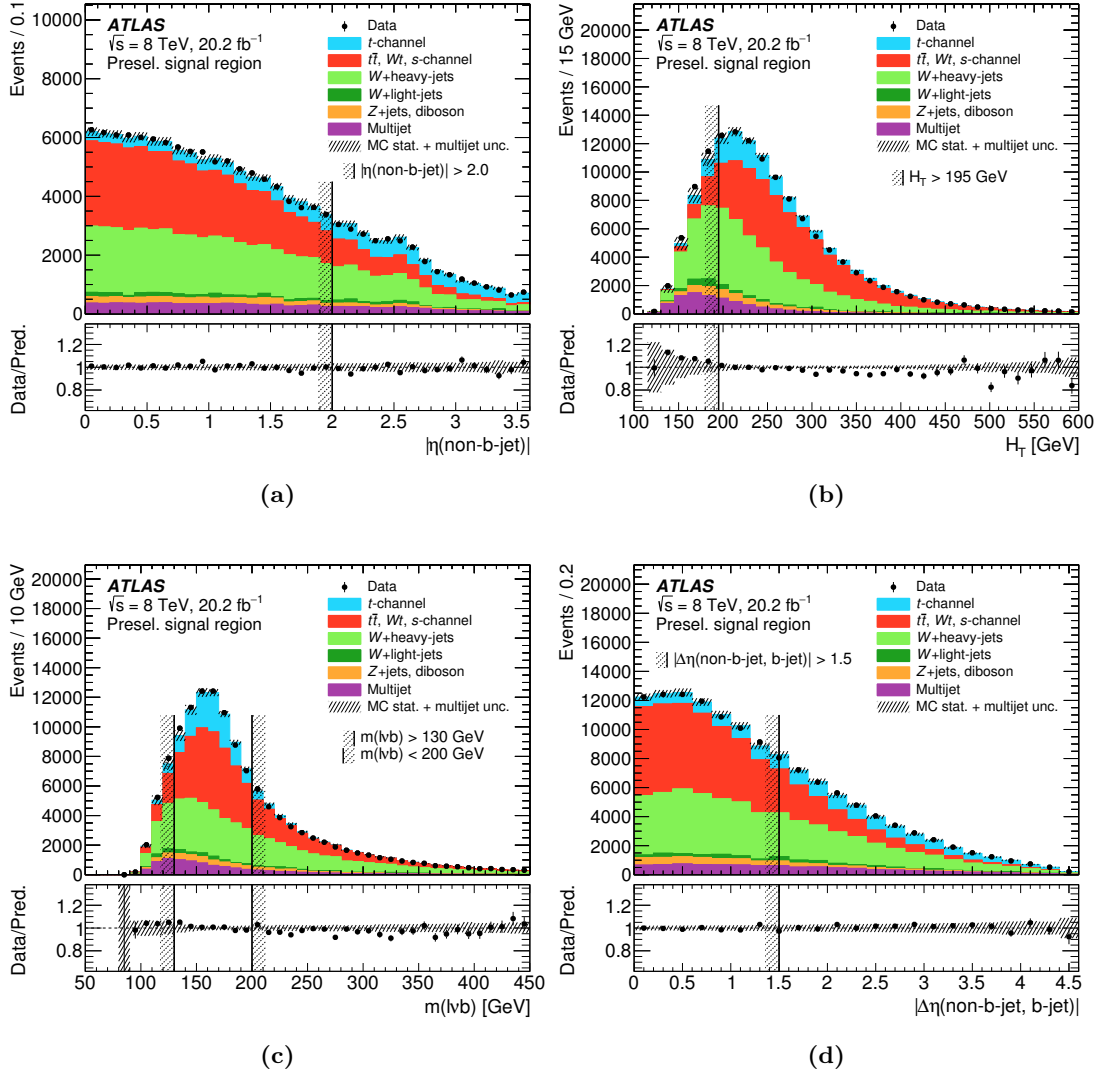
Figure 3. Distributions of (a) |\eta(\text{non-}b\text{-jet})| , (b) the scalar sum of the p_T of all final-state objects, H_T , (c) reconstructed top-quark mass, m(l\nu b) , and (d) |\Delta\eta(\text{non-}b\text{-jet}, b\text{-jet})| in the signal preselected region for the electron and muon channels merged. The prediction is compared to data, shown as the black points with statistical uncertainties. The multijet background is estimated using data-driven techniques, while contributions from simulated W +jets, top-quark backgrounds and t -channel event samples are normalised to the results of a maximum-likelihood fit to event yields in the signal and control regions. The uncertainty bands correspond to the uncertainties due to the size of the simulated event samples added in quadrature with the data-driven normalisation uncertainty of 70% estimated for the multijet contribution. The lower plots show the ratio of data to prediction in each bin. The regions excluded by the selection criteria are shown by vertical black lines and dashed areas.
