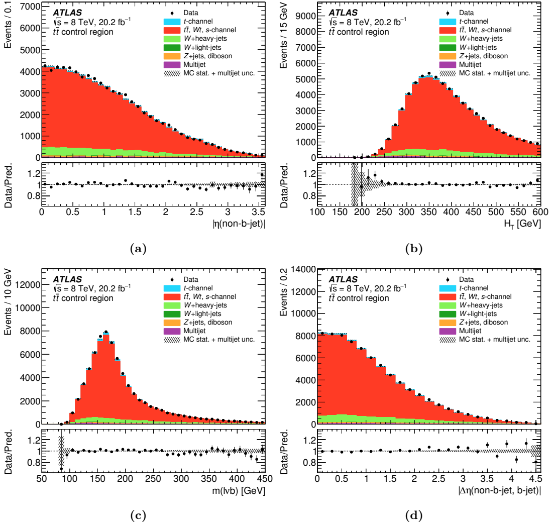
Figure 4. Distributions of (a) |\eta(\text{non-}b\text{-jet})| , (b) the scalar sum of the p_T of all final-state objects, H_T , (c) reconstructed top-quark mass, m(\ell\nu b) , and (d) |\Delta\eta(\text{non-}b\text{-jet}, b\text{-jet})| in the t\bar{t} control region for the merged electron and muon channels. The multijet background is estimated using data-driven techniques, while contributions from simulated W +jets, top-quark backgrounds and t -channel event samples are normalised to the results of a maximum-likelihood fit to event yields in the signal and control regions. The uncertainty bands correspond to the uncertainties due to the size of the simulated event samples added in quadrature with the data-driven normalisation uncertainty of 70% estimated for the multijet contribution. The lower plots show the ratio of data to prediction in each bin.
