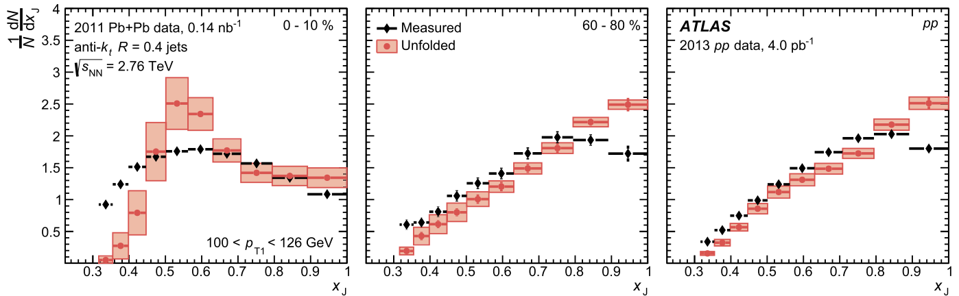
Fig. 5. The (1/N)dN/dx_J distributions for R = 0.4 jets before (black) and after (red) unfolding for the 100 < p_{T1} < 126 GeV interval for the Pb+Pb 0–10% (left) and Pb+Pb 60–80% (middle) centrality ranges and for pp collisions (right). Statistical uncertainties are indicated by vertical error bars (not visible in most cases). Systematic uncertainties in the unfolded result are indicated by the red shaded boxes. (For interpretation of the references to colour in this figure, the reader is referred to the web version of this article.)
