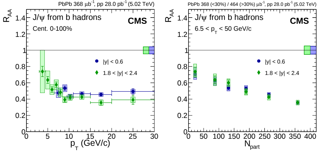
Figure 9: Nuclear modification factor of J/\psi mesons from b hadrons (nonprompt J/\psi ) as a function of dimuon p_T (left) and N_{part} (right) and in the mid- and most forward rapidity intervals. For the results as a function of N_{part} the most central bin corresponds to 0–10%, and the most peripheral one to 50–100%. The bars (boxes) represent statistical (systematic) point-by-point uncertainties. The boxes plotted at R_{AA} = 1 indicate the size of the global relative uncertainties.
