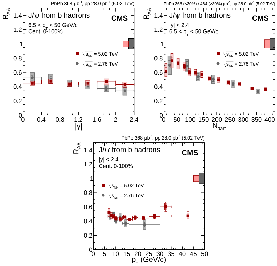
Figure 8: Nuclear modification factor of J/\psi mesons from b hadrons (nonprompt J/\psi ) as a function of dimuon rapidity (upper left), N_{\text{part}} (upper right) and dimuon p_T (lower) at \sqrt{s_{\text{NN}}} = 5.02 TeV. For the results as a function of N_{\text{part}} the most central bin corresponds to 0–5%, and the most peripheral one to 70–100%. Results obtained at 2.76 TeV are overlaid for comparison [11]. The bars (boxes) represent statistical (systematic) point-by-point uncertainties. The boxes plotted at R_{\text{AA}} = 1 indicate the size of the global relative uncertainties.
