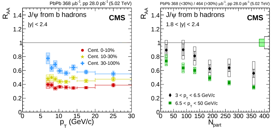
Figure 10: Nuclear modification factor of J/\psi mesons from b hadrons (nonprompt J/\psi ). Left: as a function of dimuon p_T in three centrality bins. Right: as a function of N_{part} at moderate and high p_T , in the forward 1.8 < |y| < 2.4 range. For the results as a function of N_{part} the most central bin corresponds to 0–10%, and the most peripheral one to 50–100%. The bars (boxes) represent statistical (systematic) point-by-point uncertainties. The boxes plotted at R_{AA} = 1 indicate the size of the global relative uncertainties.
