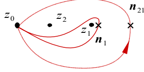
Figure 3: A set of auxiliary contours for the braiding calculation.
