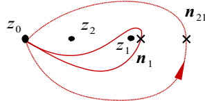
Figure 7: A set of auxiliary contours for the braiding calculation.
