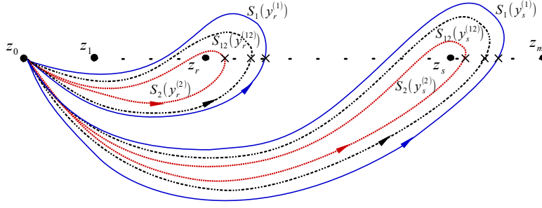
Figure 1: Nested non-intersecting and non-self-intersecting multi-contours for integration over screening currents associated with different vertex operators. The multi-contours around a puncture and which associated with a particular screening charge are depicted collectively by one loop.
