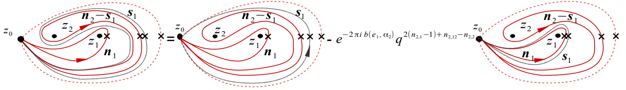
Figure 8: Deformation of the outermost of the contours encircling z_2 .
