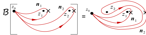
Figure 6: Braiding of two generic multi-contours.
