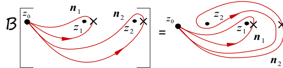
Figure 2: Braiding of two generic multi-contours. The collections of contours associated with general products of screening charges are depicted here are simple loops around the punctures.
