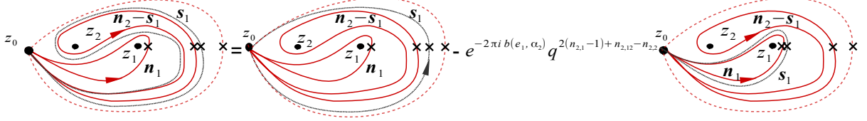
Figure 4: Deformation of the outermost of the contours encircling z_2 representing a step in the passage to linear combinations of the contour depicted in Figure 3.
