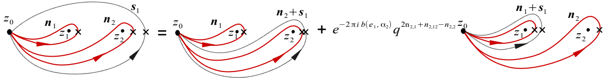
Figure 5: Decomposition of a simple contour associated with the root e_1 around two punctures into contours enclosing only one of the punctures. This decomposition represents the co-product \Delta(\mathbf{f}_1) = 1 \otimes \mathbf{f}_1 + \mathbf{f}_1 \otimes \mathbf{k}_1^{-1} .
