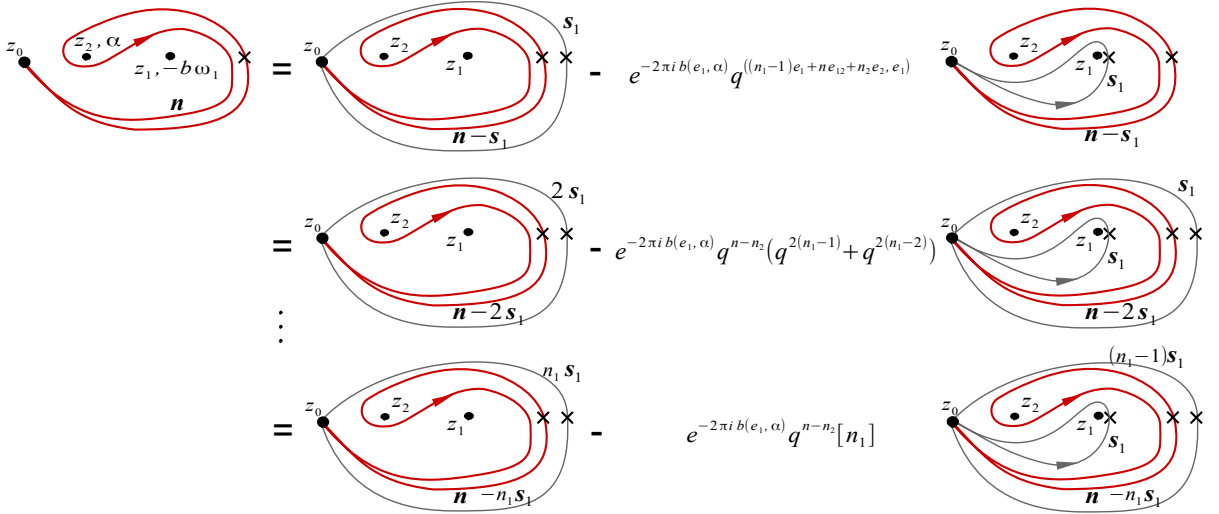
Figure 9: Example illustrating how quantum numbers arise in the braiding calculation.
