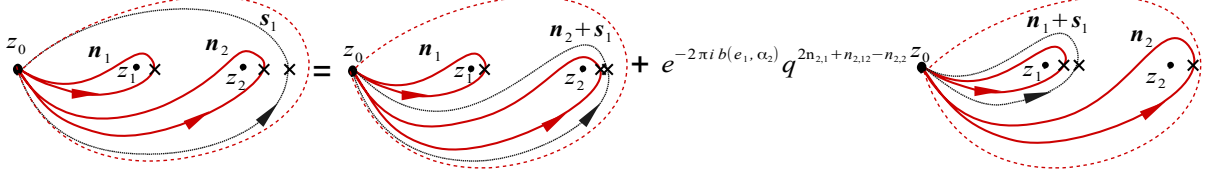
Figure 10: Decomposition of a simple contour associated with the root e_1 around two punctures into contours enclosing only one of the punctures.
