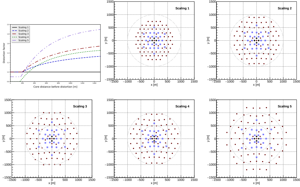
Figure 1: Top-left: Radially symmetric distortion factors for the five different scalings in prod3 CTA South layouts, as a function of the core distance before this distortion. Top-right to bottom-right: an example of the scalings for the Paranal site for one of the studied layouts. LSTs positions are shown with black circles, MSTs with blue squares, and SSTs with filled red circles.
