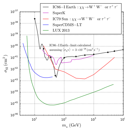
Fig. 8 Upper limits at 90% confidence level on \sigma_{\chi-N}^{\text{SI}} as a function of the WIMP mass assuming a WIMP annihilation cross section of \langle\sigma_A v\rangle = 3 \times 10^{-26} cm 3 s -1 . For WIMP masses above the rest mass of the W bosons, annihilation into W^+W^- is assumed and annihilation into \tau^+\tau^- for lower masses. Systematic uncertainties are included. The result is compared to the limits set by SuperCDMSlite [6], LUX [5], Super-K [22] and by a Solar WIMP analysis of IceCube in the 79-string configuration [24]. The displayed limits are assuming a local dark matter density of \rho_\chi = 0.3 GeV cm -3 . A larger density, as suggested e.g. by [59], would scale all limits linearly
