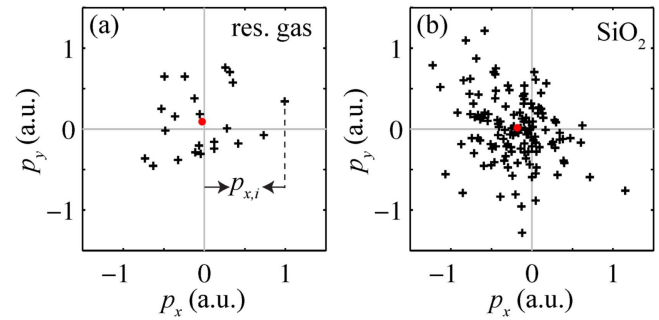
Figure 6. Post-processed single-shot momentum images (projected along p_z ) of the electron emission for (a) residual gas and (b) \text{SiO}_2 nanoparticles obtained in the XUV-NIR streaking experiments. The red dots show averages of the momentum distributions. The asymmetry in the photoelectron momentum distribution along the laser propagation direction ( p_x ) originates from preferential absorption of XUV light on the front side of the nanoparticle (shadowing).
