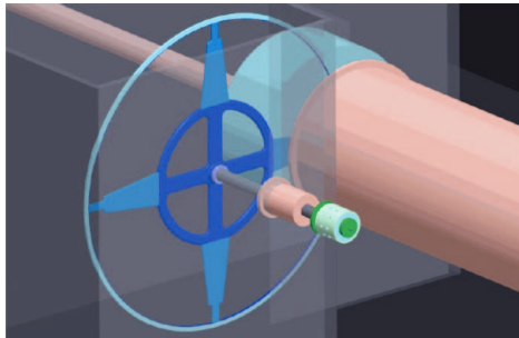
Figure 3: Layout of the positron target. The target is a rotating disc with a diameter of 1 m in order to reduce local stress. Picture taken from [4].
