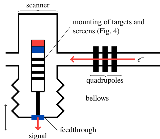
Figure 5: Arrangement to irradiate multiple targets at SF 35.
