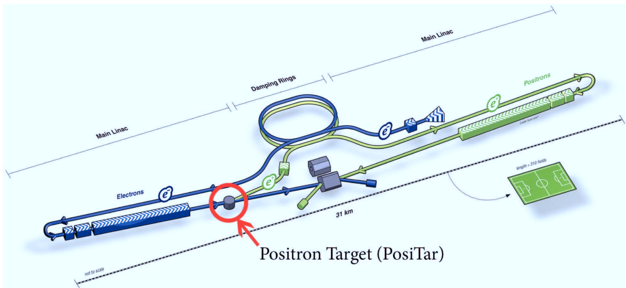
Figure 2: Schematic sketch of the ILC -beam line. [3]
