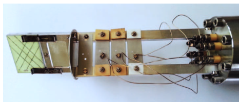
Figure 4: Holder for multiple targets. Two screens on top of the targets are needed for beam optimization. The multiple feedthroughs/wires serve to measure the temperatures and currents on the different targets.
