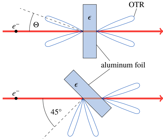
Figure 6: Scheme of emitted OTR (blue) at the aluminum foil perpendicular to the beam and at an angle of 45^\circ . In the latter case, OTR can be observed easily at an angle of \approx 90^\circ . [6]
