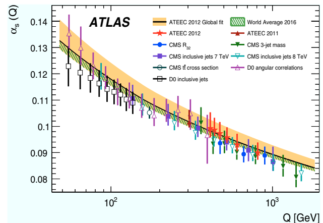
Fig. 11 Comparison of the values of \alpha_s(Q) obtained from fits to the ATEEC functions at the energy scales given by \langle H_{T2} \rangle / 2 (red star points) with the uncertainty band from the global fit (orange full band) and the 2016 world average (green hatched band). Determinations from other experiments are also shown as data points. The error bars, as well as the orange full band, include all experimental and theoretical sources of uncertainty. The strong coupling constant is assumed to run according to the two-loop solution of the RGE
