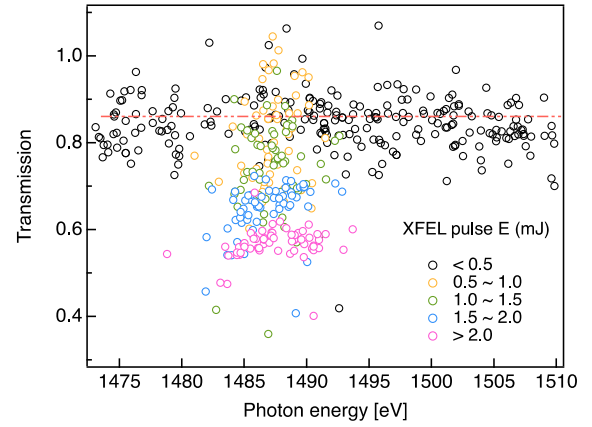
FIG. 1. Measurement of x-ray transmission through an aluminum foil target. Each circle represents the data from a single shot. The red line is the known transmission value of cold Al from the CXRO database. The peak intensities of the highest pulse energies (pink circles) correspond to \sim 10^{17} \text{ W/cm}^2 .
