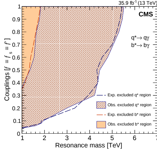
Figure 6: The observed and expected regions excluded at 95% CL for q^* and b^* production and decay, as a function of m_{q^*} , m_{b^*} and f .
