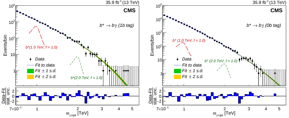
Figure 3: The \gamma + b jet invariant mass distribution in data (black points) used for the b^* analysis, after final selection for (left) 1b tag category and (right) 0b tag category. The result of the fit to the data using the parametrization defined in Eq. (2) is shown by the blue dashed curve with associated bands indicating the uncertainty. The bin-by-bin pull, (\text{Data-Fit})/(\text{stat. unc.}) , where the denominator refers to the statistical uncertainty in data, is also presented. The green and yellow bands corresponds to 1 and 2 standard deviations, respectively from the mean value. Simulations of excited b quark signals representing the expected excess of signal events over the background are shown for the 1b and 0b tag categories for the mass values of 1.0 and 2.0 TeV for f = 1.0 .
