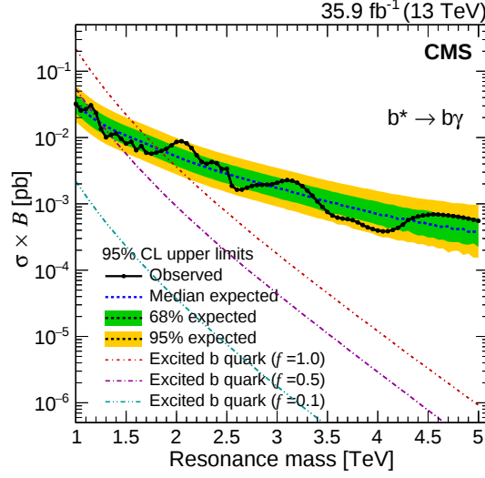
Figure 5: The observed and expected upper limits at 95% CL on \sigma \mathcal{B} as a function of the mass of the excited b quark, for f = 1.0 . The limits are compared with theoretical predictions for excited b quark production for three couplings. The inner (green) band and the outer (yellow) band indicate the regions containing 68 and 95%, respectively, of the mean limits under the background-only hypothesis.
