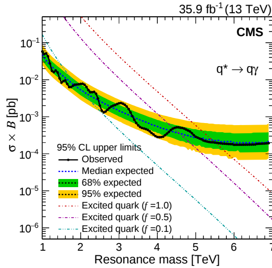
Figure 4: The observed and expected upper limits at 95% CL on \sigma \mathcal{B} as a function of the mass of the excited quark, for f = 1.0 . The limits are compared with theoretical predictions for excited quark production for three couplings. The inner (green) band and the outer (yellow) band indicate the regions containing 68 and 95%, respectively, of the mean limits under the background-only hypothesis.
