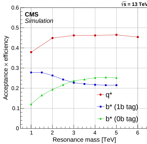
Figure 1: The product of acceptance and efficiency for q^* and b^* signals as a function of generated m_{q^*} or m_{b^*} mass, calculated using MC simulation.
