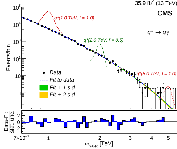
Figure 2: The \gamma + \text{jet} invariant mass distribution in data (black points) for the inclusive category used for the q^* analysis, after final selection. The result of the fit to the data using the parametrization defined in Eq. (2) is shown by the blue dashed curve with associated bands indicating the uncertainty. The bin-by-bin pull, (\text{Data-Fit})/(\text{stat. unc.}) , where the denominator refers to the statistical uncertainty in data, is also presented. The green and yellow bands corresponds to 1 and 2 standard deviations, respectively from the mean value. Simulations of excited quark signals representing the expected excess of signal events over the background are shown for the mass values of 1.0 and 5.0 TeV for f = 1.0 , and 2.0 TeV for f = 0.5 .
