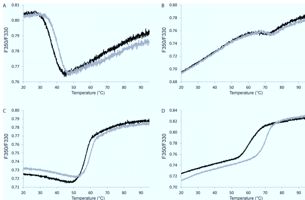
Figure 3. DSF transition curves of various IMP targets in the absence and presence of selected LLPs. Shown are the raw fluorescence data (ratio F350/F330). A) \text{PepT}_{\text{st}} in NM, B) YkoE in NM, C) hypothetical sugar transporter in LMNG, and D) GlpG in NG. Experiments were performed with IMPs \pm 2.5 mM LLP (in 4% DMSO) by using a heating rate of 1^\circ\text{C min}^{-1} .
