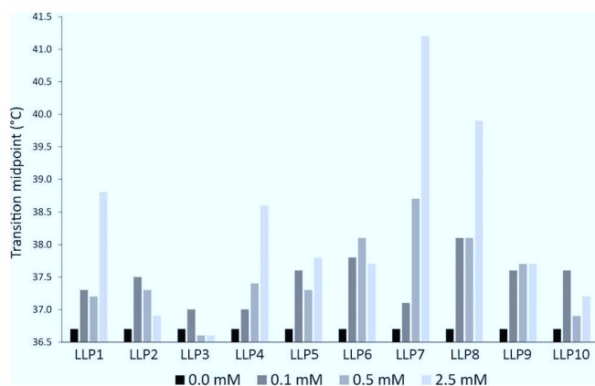
Figure 4. Concentration dependence of the observed transition midpoint. DSF curves were acquired for 1 \text{ mg mL}^{-1} \text{PepT}_{\text{st}} in 0.4% NM in the presence of different concentrations (0–2.5 mM) of various LLPs.
