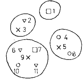
figure 1. Clusters of labelled vertices of different colour.
