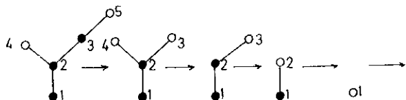
figure 3 How to trim a tree and straighten its branches. (The last dot represents a single constituent of the \ell -vertex \alpha_1 .)
