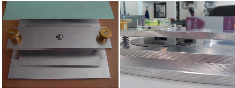
Figure 11.6: Picture of the jig to align and fix the NanoPorts on the prototypes (left) and of the alignment process with a NanoPort mounted in the jig (right).
