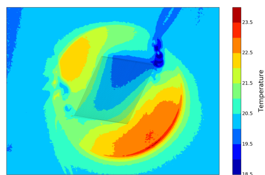
(d) Experiment with the anodic bonded sample with a flow rate of 30 \text{ ml min}^{-1} .
