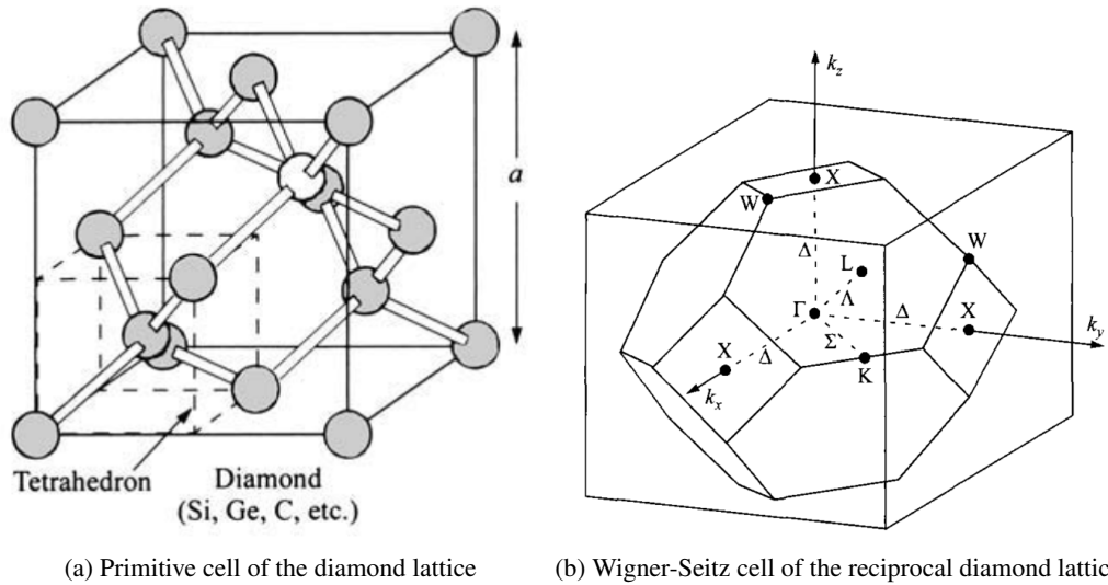
Figure 3.1: The primitive cell of silicon with the lattice constant a shown in figure a) and the Wigner-Seitz cell (first Brillouin zone) of the reciprocal lattice shown in figure b).
