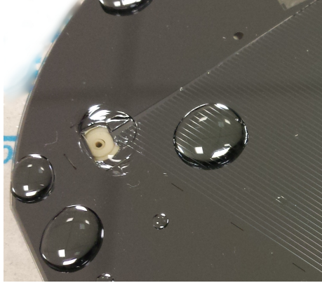
Figure 11.7: Broken silicon wafer due to a pressure increase to 31 bar.
