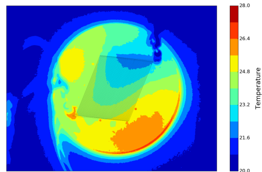
(b) Experiment with the anodic bonded sample with a flow rate of 10 \text{ ml min}^{-1} .
