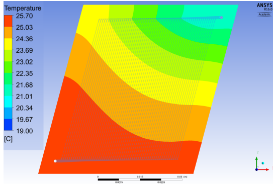
(a) Simulation with a flow rate of 10 \text{ ml min}^{-1}
