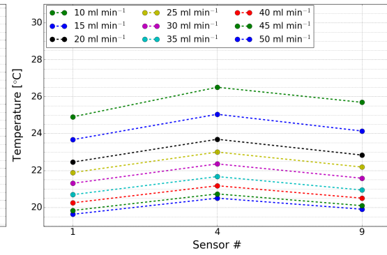
(b) Line 3 on the eutectic bonded sample.
