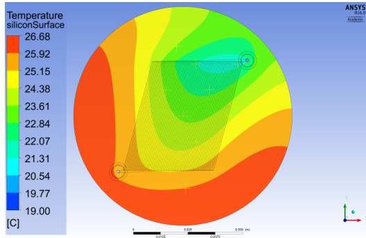
(a) Simulation with the anodic bonded sample with a flow rate of 10 \text{ ml min}^{-1} .
