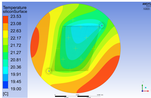
(c) Simulation with the anodic bonded sample with a flow rate of 30 \text{ ml min}^{-1} .
