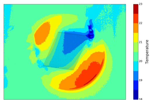
(f) Experiment with the anodic bonded sample with a flow rate of 50 \text{ ml min}^{-1} .
