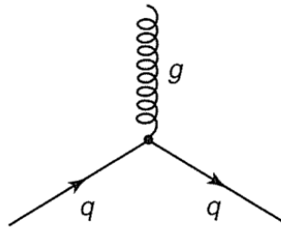
Figure 2.3: One fundamental process in QCD. A quark emits (or absorbs) a gluon [6].
