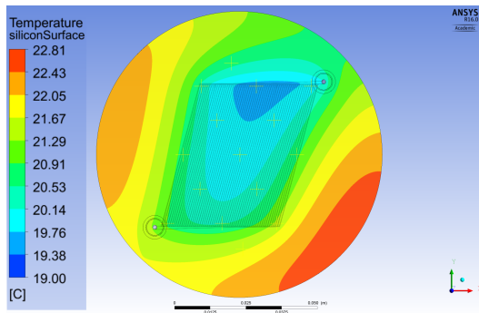
(e) Simulation with the anodic bonded sample with a flow rate of 50 \text{ ml min}^{-1} .
