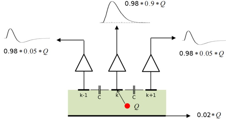
Figure 7.3: Scheme of the capacitive crosstalk effect in a micro strip detector. Fake signals appear on the neighboring strips k-1 and k+1 after an ionising event produced a signal on strip k . In total 2% of the charge is transferred to the backplane of the sensor and 5% to each neighboring strip [51].
