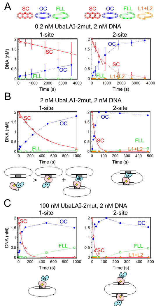
Figure 6. UbaLAI-2mut reactions on plasmids with one and two recognition sites. As in Figure 3, cartoons above the graphs depict DNA forms that can exist during UbaLAI reactions on plasmids with one and two UbaLAI sites. (A) Steady-state reactions, performed with 2 nM DNA and 0.2 nM UbaLAI-2mut. Continuous lines are linear fits to the initial SC DNA cleavage data that yielded DNA cleavage rates (optimal value \pm SEM) of 0.00018 \pm 0.00008 \text{ nM s}^{-1} and 0.0016 \pm 0.0006 \text{ nM s}^{-1} for the 1-site and 2-site plasmids, respectively. (B) Reactions performed with equimolar enzyme and DNA (2 nM each) concentrations. Continuous lines are single exponential fits to the SC DNA cleavage data that yielded the observed first order rate constants of 0.0025 \pm 0.0002 \text{ s}^{-1} and 0.034 \pm 0.004 \text{ s}^{-1} for the 1-site and the 2-site plasmids, respectively. (C) Reactions performed under enzyme excess conditions (100 nM UbaLAI-2mut, 2 nM DNA). Single exponential fits yielded the observed first order rate constants of 0.015 \pm 0.002 \text{ s}^{-1} and 0.07 \pm 0.01 \text{ s}^{-1} for the 1-site and the 2-site plasmids, respectively. Cartoons below the graphs in panels (B) and (C) schematically depict the protein-DNA complexes formed by UbaLAI-2mut with 1- and 2-site plasmids.
