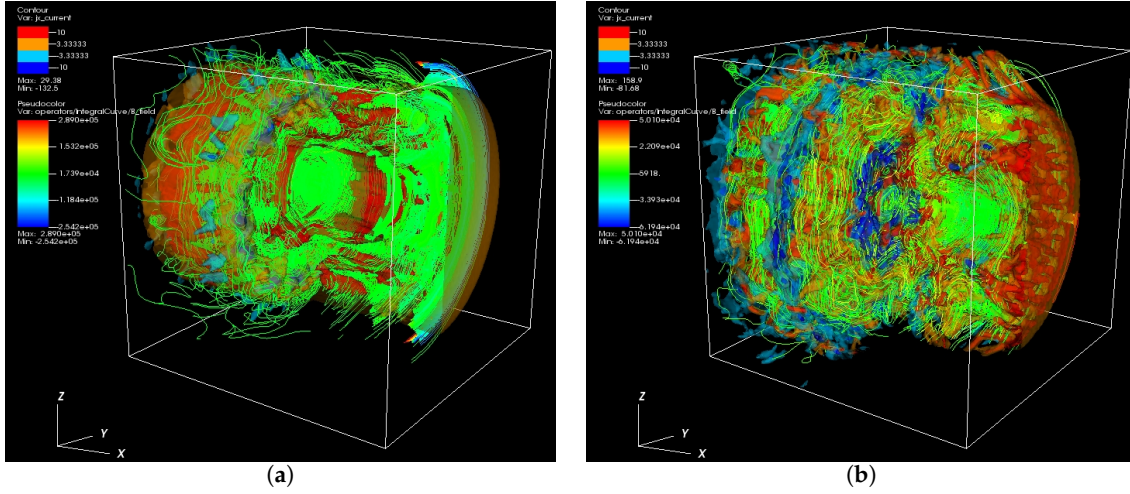
Figure 2. Panels show 3D iso-surface plots of the current ( J_x ) of jet electrons for e^- - p^+ (a) and e^\pm (b) jets with r_{\text{jet}} = 80\Delta at time t = 500\omega_{pe}^{-1} . The lines show the magnetic field stream lines in the quadrant of the front part of the jets. Color scales for the contour (upper left) for (a,b) are red: 10; orange: 3.33; right blue: -3.33; blue: -10. The color scales of streaming lines are (a) (2.89, 1.53, 0.174, -1.2, -2.54) \times 10^5 , and (b) (5.01, 2.21, -0.592, -3.39, -6.19) \times 10^4 .
