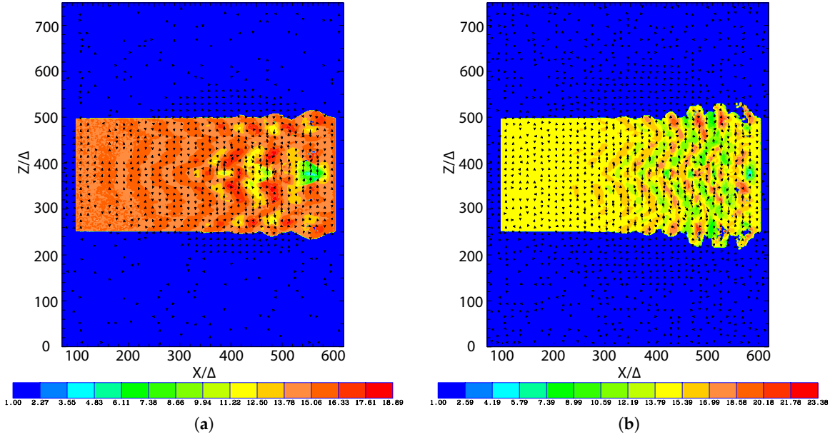
Figure 3. Panels (a,b) show 2D plot of the Lorentz factor of jet electrons for e^- - p^+ (a) and e^\pm (b) jets with r_{\text{jet}} = 120\Delta at time t = 500\omega_{pe}^{-1} . The arrows (black spots) show the magnetic fields in the x - z plane.
