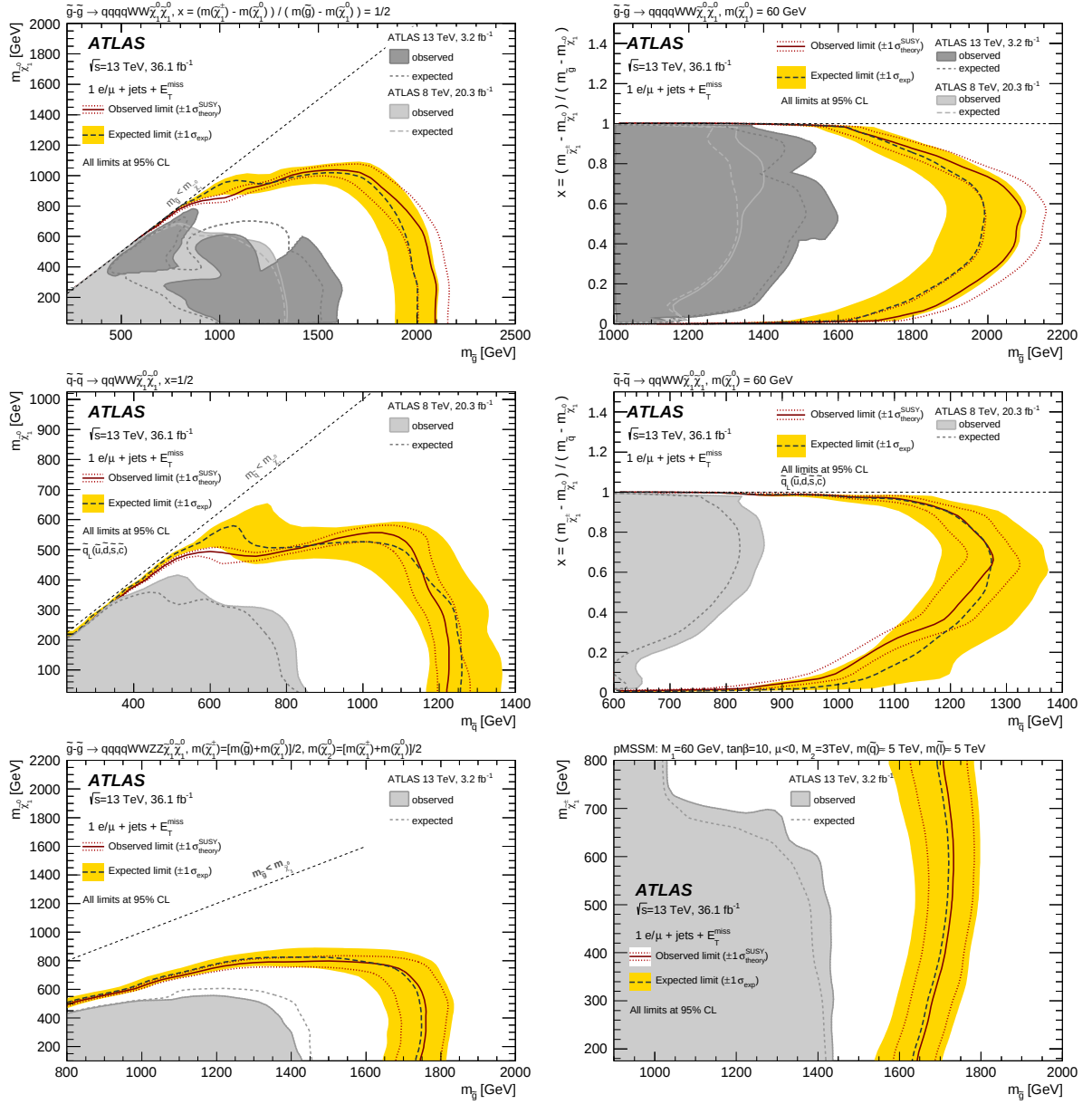
Figure 10: Exclusion contours for gluino one-step x = 1/2 (top left), gluino one-step variable- x (top right), squark one-step x = 1/2 (middle left) and squark one-step variable- x (middle right), gluino two-step (bottom left), and the pMSSM scenario (bottom right). The red solid line corresponds to the observed limit with the red dotted lines indicating the \pm 1\sigma variation of this limit due to the effect of theoretical scale and PDF uncertainties in the signal cross-section. The dark gray dashed line indicates the expected limit with the yellow band representing the \pm 1\sigma variation of the median expected limit due to the experimental and theoretical uncertainties. For reference, exclusion bounds from previous searches with 20.3 \text{ fb}^{-1} at 8 TeV center-of-mass energy [28] and 3.2 \text{ fb}^{-1} at 13 TeV center-of-mass energy [22, 30] are overlaid where applicable by the gray area (the observed limit is shown by the solid line, while the dashed line shows the expected limit).
