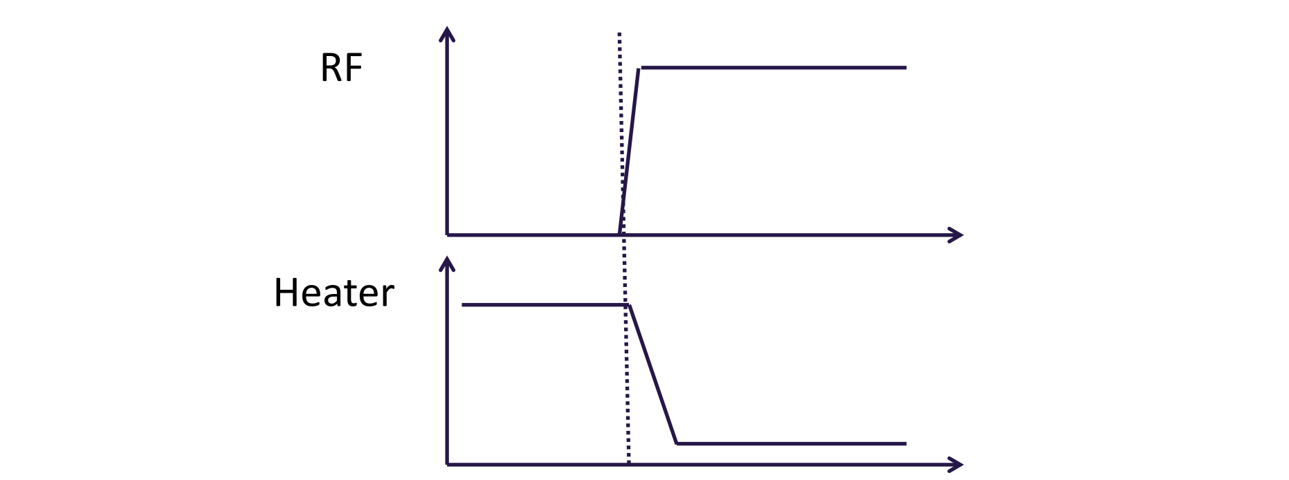
Figure 1: Heater power decreasing while RF power increases and thus dissipates the same amount of heat into the LHe bath. The overall energy balance stays constant.
