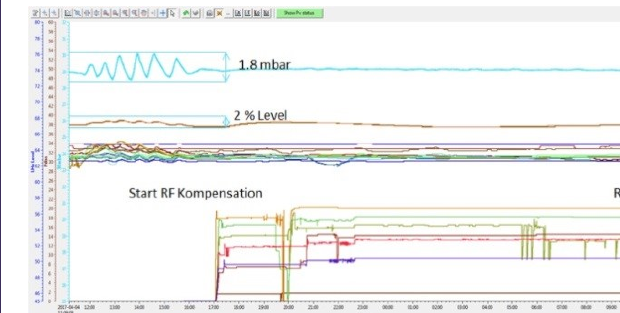
Figure 4: First run with heat load compensation switched on. And first RF trip the next day.
