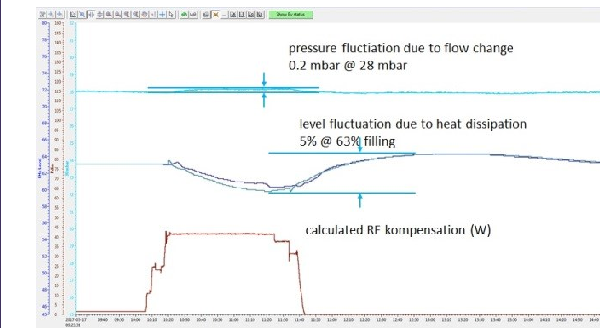
Figure 5: 'Soft quench' of just one cavity can cause major problems in a cryo string.
