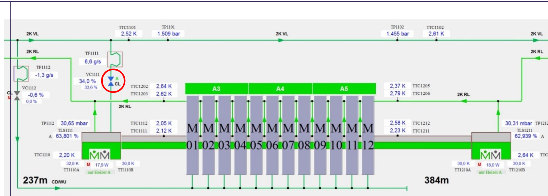
Figure 2: A cryo string in the XFEL consists of twelve cryo modules. The main control loop is configured to keep the LHe level constant by setting the JT valve accordingly.
