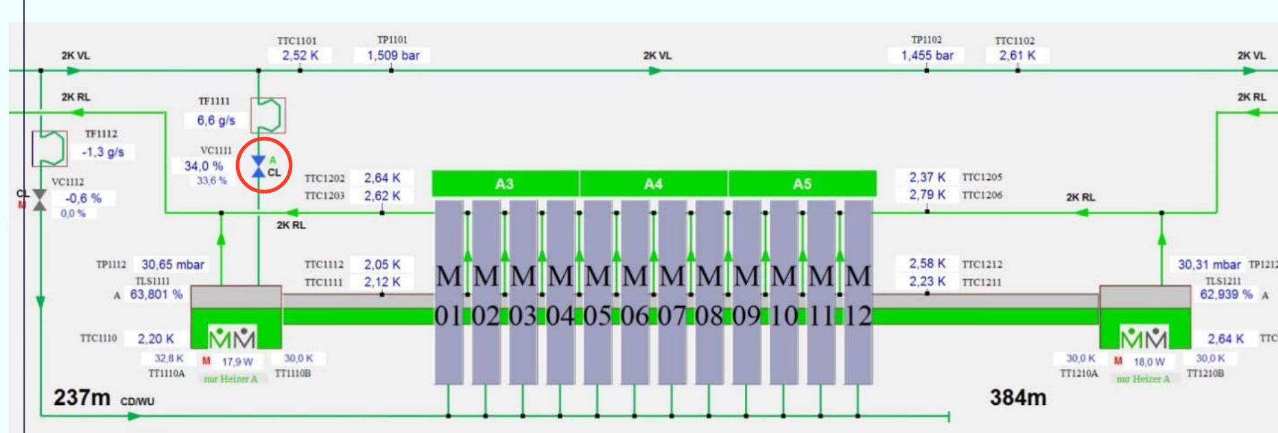
Figure 2: A cryo string in the XFEL consists of twelve cryo modules. The main control loop is configured to keep the LHe level constant by setting the JT valve accordingly.
