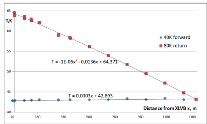
Figure 9. Temperature profiles along XFEL linac.
