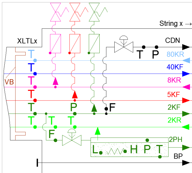
Figure 5. Flow scheme of FC1-3.
