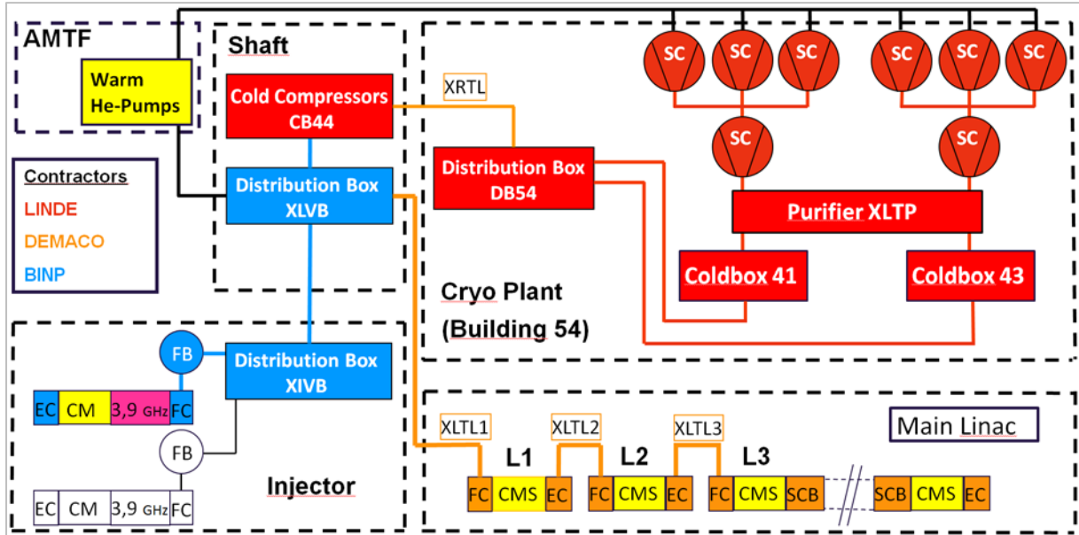
Figure 1. Layout of XFEL cryogenic components.
