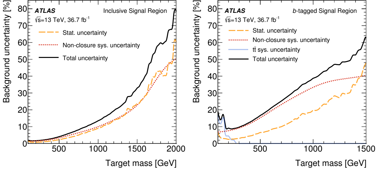
Figure 6: The uncertainty in the data-driven background estimate in the inclusive (left) and b -tagged (right) signal regions, computed in the m_{\text{avg}} mass windows defined for different target masses. The uncertainty arising from the non-closure in the validation region is shown with a red short-dashed line and compared with the statistical uncertainty of the data-driven prediction shown as an orange dashed line. The additional uncertainty in the MC estimate of the top background in the b -tagged signal region is shown as a dotted blue line. The total uncertainty, obtained by adding in quadrature the different components, is indicated by a black solid line.
