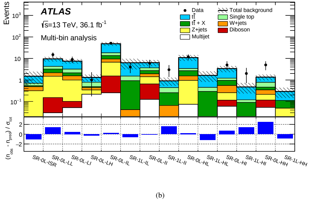
Figure 9: Results of the background-only fit extrapolated to the SRs for (a) the cut-and-count and (b) the multi-bin analyses. The data in the SRs are not included in the fit. The upper panel shows the observed number of events and the predicted background yield. All uncertainties defined in Section 7 are included in the uncertainty band. The background category t\bar{t} + X includes t\bar{t}W/Z , t\bar{t}H and t\bar{t}t\bar{t} events. The lower panel shows the pulls in each SR.
