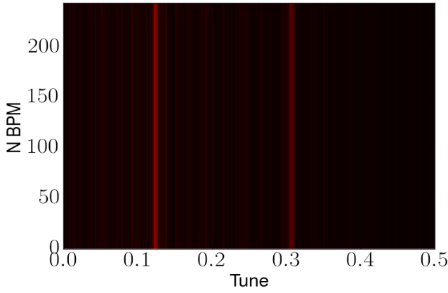
Figure 5: Y spectrum, corresponding to horizontal excitation of 6 mm and vertical excitation of 3 mm.
