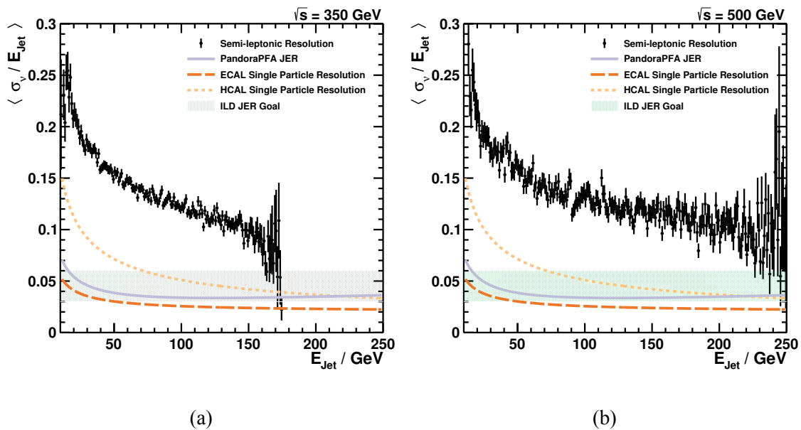
Figure 7.14 – Average relative uncertainty on the jet energy due to the semi-leptonic correction as a function of the jet energy for events with semi-leptonic decays. The intrinsic energy resolutions of the calorimeters for single particles are shown for comparison. The horizontal band represents the target region of the jet energy resolution at ILD. The solid line indicates the jet energy resolution of the PandoraPFA [40].
