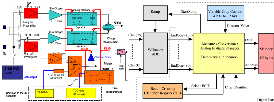
Figure 9.1 – Schematic diagram of one channel of the SPIROC ASIC [111].
