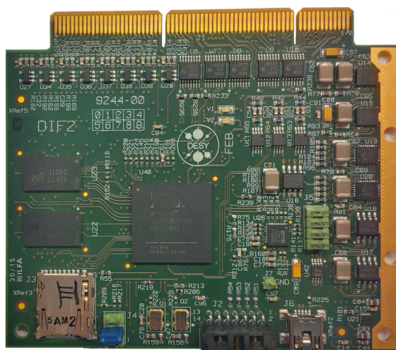
Figure 10.3 – The Detector Interface (DIF) board for CALICE scintillator calorimeters.
