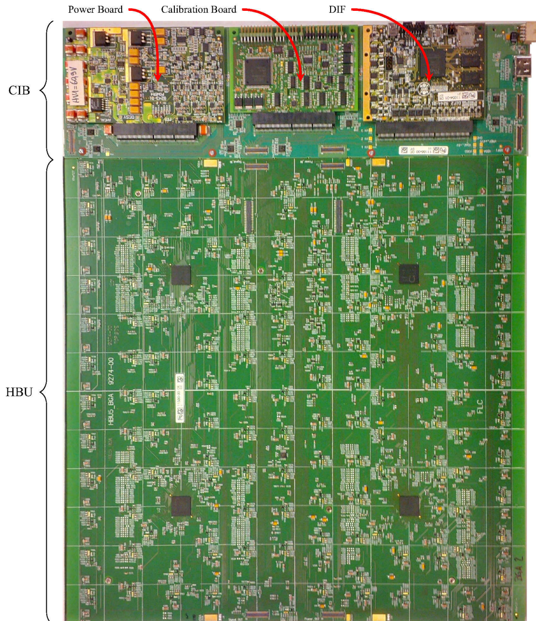
Figure 9.3 – A HCAL Base Unit (HBU) with Central Interface Board (CIB) and power, calibration and Detector Interface (DIF) boards. Each of the white squares on the HBU depicts the area of one scintillator tile which is mounted on the rear side of the HBU. The four black squares are the read-out ASICs.
