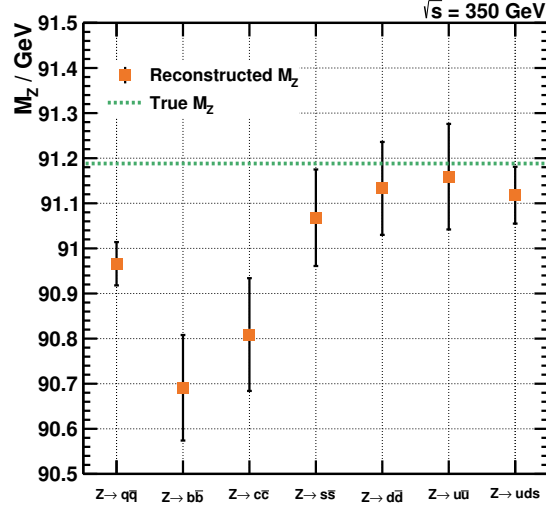
Figure 8.3 – Reconstructed Z boson mass using the \chi^2 -minimisation method for Z \rightarrow q\bar{q} , Z \rightarrow b\bar{b} , Z \rightarrow c\bar{c} , Z \rightarrow s\bar{s} , Z \rightarrow d\bar{d} , Z \rightarrow u\bar{u} and Z \rightarrow uds ( Z boson decays to any of the light quark pairs) processes. While the reconstructed mass of the Z \rightarrow d\bar{d} and Z \rightarrow u\bar{u} samples are in agreement with the simulation input mass of Z boson, the reconstructed masses of Z \rightarrow c\bar{c} and Z \rightarrow b\bar{b} data samples are underestimated by \sim 500\text{MeV} and \sim 400\text{MeV} , respectively.
