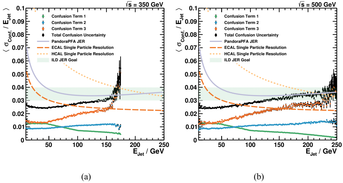
Figure 7.10 – Average relative uncertainty on the jet energy due to the confusion as a function of the jet energy. The intrinsic energy resolutions of the calorimeters for single particles are shown for comparison. The horizontal band represents the target region of the jet energy resolution at ILD. The solid line indicates the jet energy resolution of the PandoraPFA [40].
