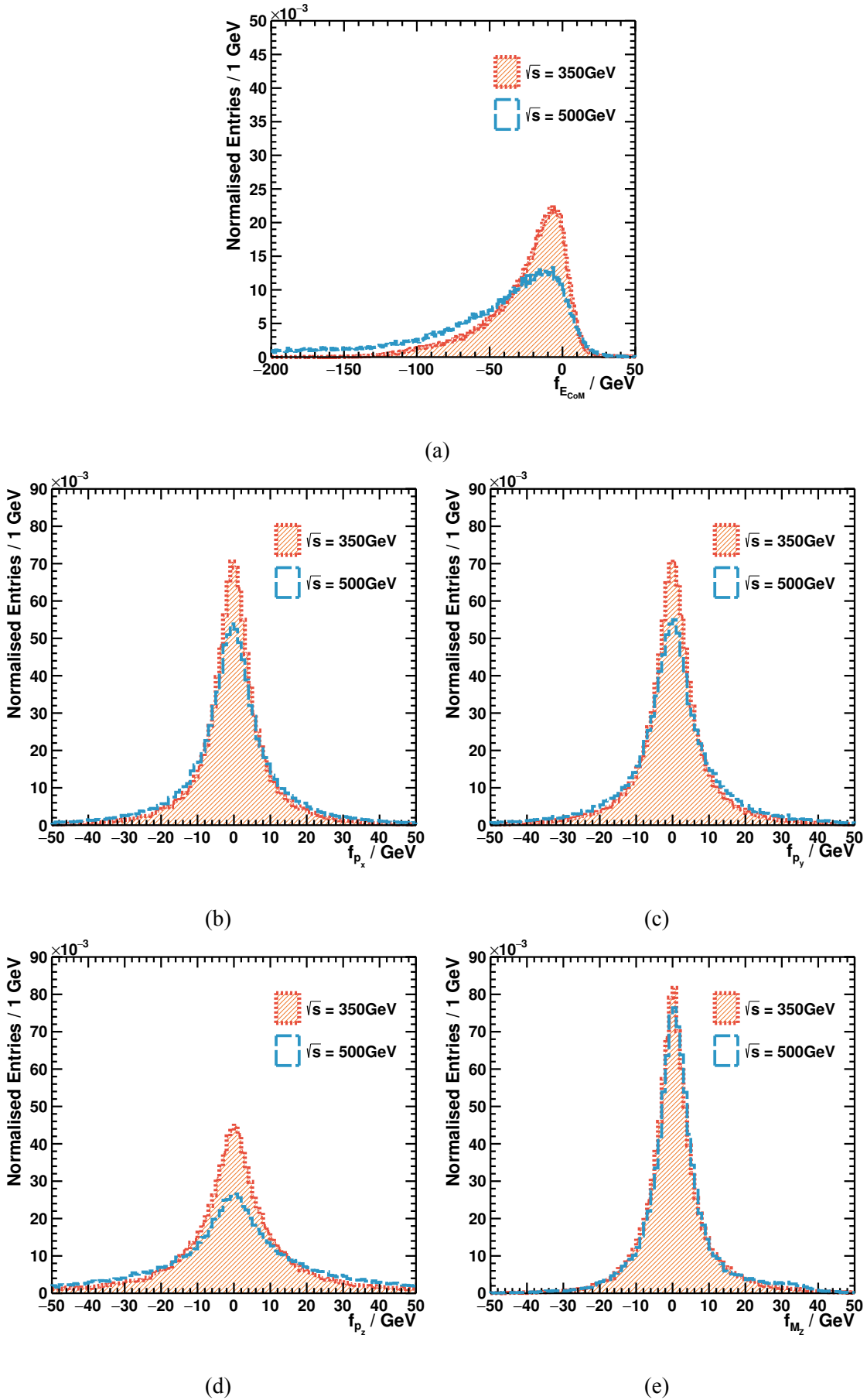
Figure 8.4 – Distributions of the initial values of various constraints used in kinematic fitting for the centre-of-mass energies of 350 GeV and 500 GeV.
