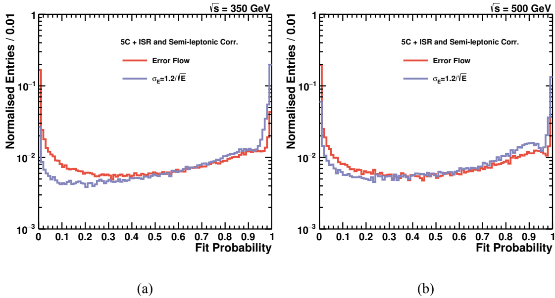
Figure 8.12 – Comparison of the kinematic fit probability using the jet-specific energy uncertainty and a fixed uncertainty of 120\%/\sqrt{E} . The analysis is performed on the MC samples of 350 GeV and 500 GeV centre-of-mass energy with 5C fit hypothesis with ISR and semi-leptonic corrections.
