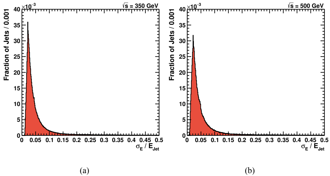
Figure 7.15 – Distribution of the relative total jet energy resolution obtained using the error flow method for the centre-of-mass energies of 350 GeV and 500 GeV.
