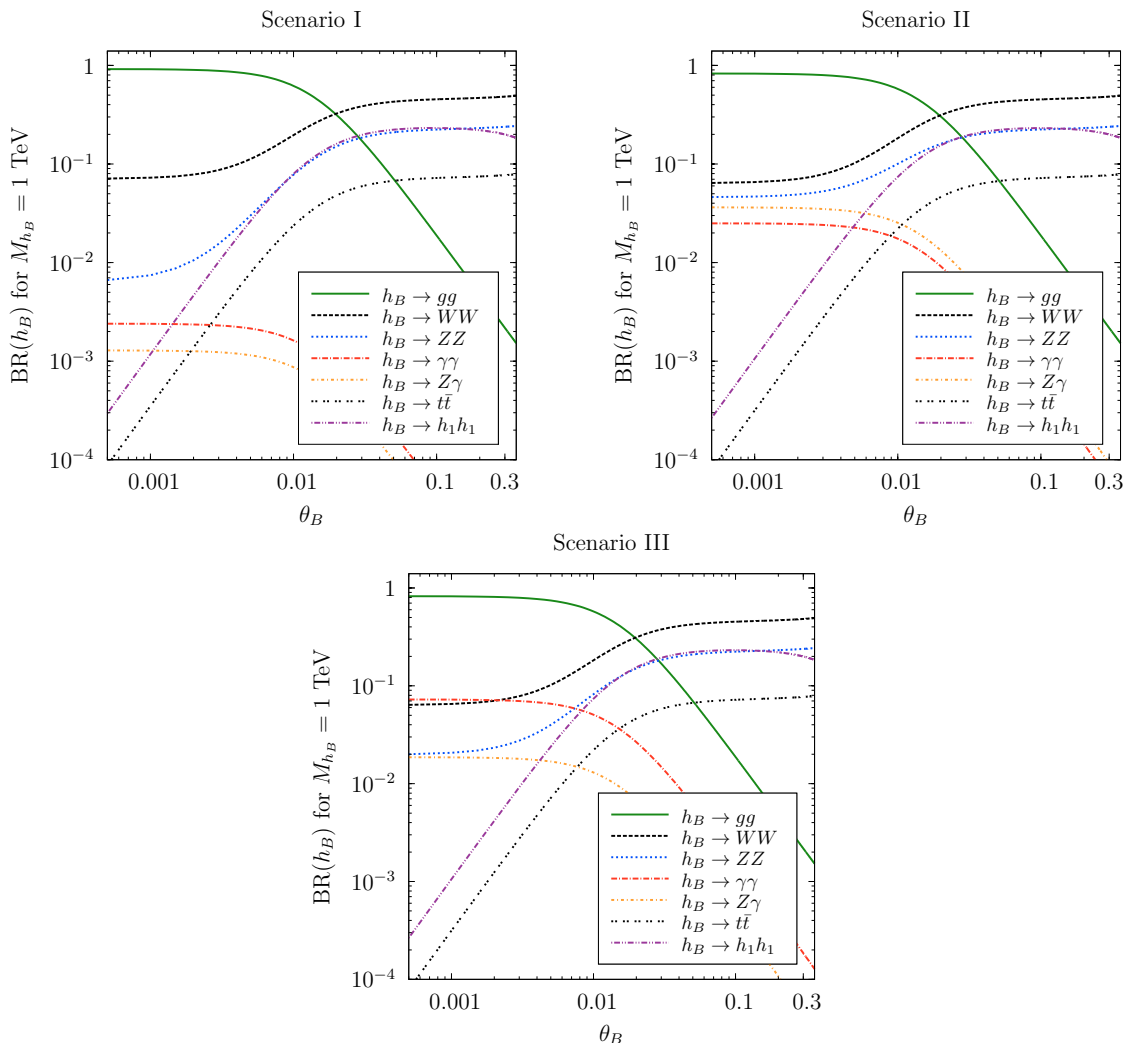
Figure 1. Branching ratios of the baryonic Higgs as a function of the mixing angle \theta_B assuming only decays into SM particles. The vector-like quarks are assumed to be heavy and we use v_B = 2 TeV and M_{h_B} = 1 TeV.
