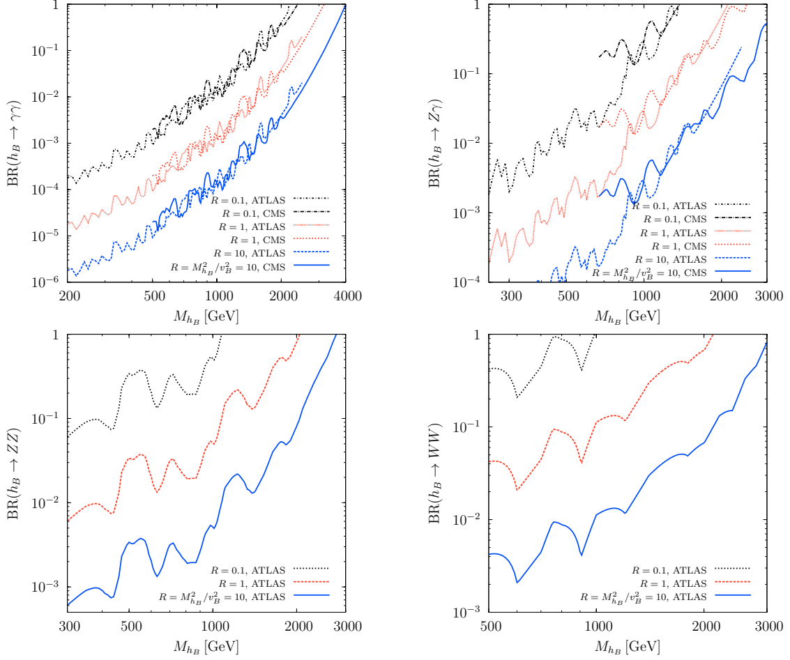
Figure 3. Constraints on the branching ratios of h_B into two photons [26, 27], Z\gamma [28, 29], ZZ [30], and WW [31] for different choices of the ratio between mass and vev of the baryonic Higgs field. In the plots n_f = 3 .
