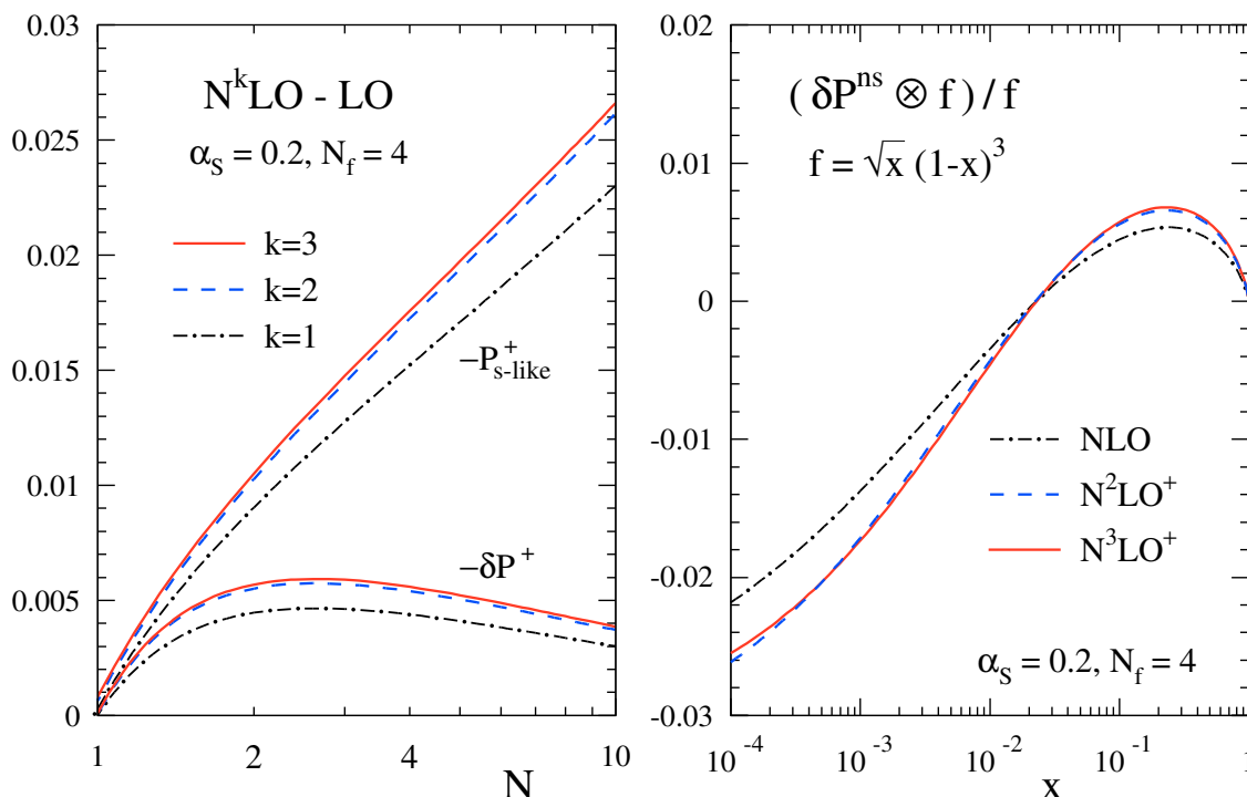
Figure 13. The perturbative expansion of the difference \delta P^+ = P_{\text{ns}, \sigma=1}^+ - P_{\text{ns}, \sigma=-1}^+ of the time-like ( \sigma = 1 ) and space-like ( \sigma = -1 ) non-singlet + splitting functions. Left: results in Mellin-space, compared to beyond-LO contributions in the space-like case. Right: convolution with the schematic input shape (5.6).
