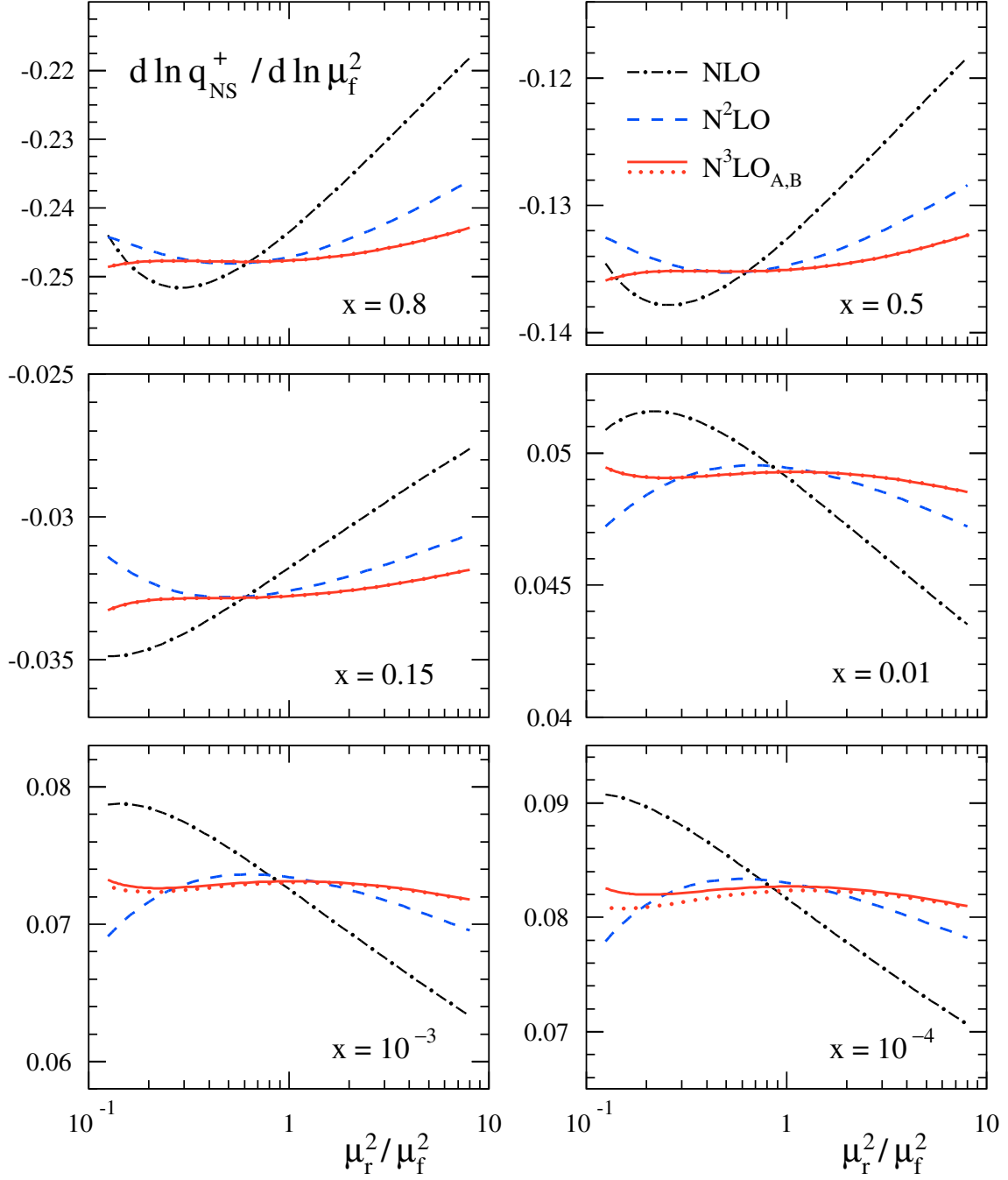
Figure 9. The dependence of the NLO, NNLO and N 3 LO predictions for \dot{q}_{\text{ns}}^+ \equiv d \ln q_{\text{ns}}^+ / d \ln \mu_f^2 on the renormalization scale \mu_r , at six typical values of x for the initial conditions (5.6) and (5.7). The effect of the remaining uncertainty of the four-loop splitting function P_{\text{ns}}^{(3)+} , indicated by the difference of the solid and dotted curves, is practically invisible except for the last two panel.
