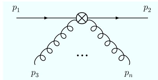
Figure 1. Vertices with additional gluons arising from the operators O_{\{\mu_1, \dots, \mu_N\}}^{\text{ns}} in perturbative QCD. Vertices with up to L gluons need to be considered at L loops at Mellin moments N > L .
