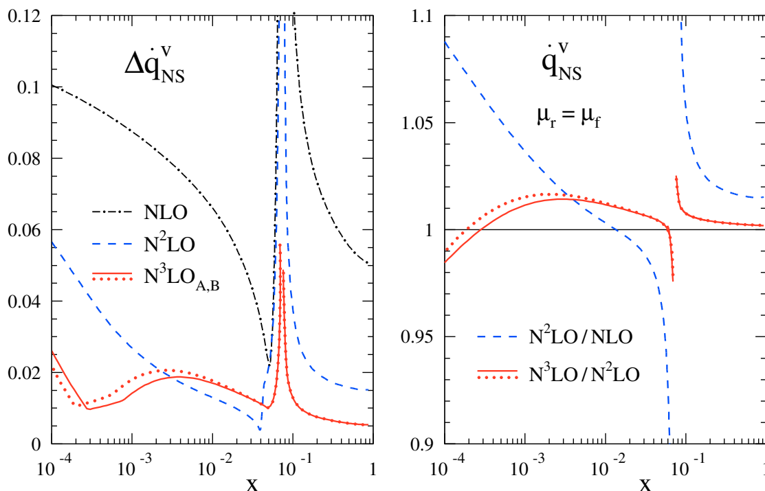
Figure 12. As figures 10 and 11, but for the total (flavour-summed) valence quark distribution q_{\text{ns}}^v . Here and in figures 10 and 11 the spikes close to x = 0.07 reflect the sign-changes of \dot{q}_{\text{ns}}^i and do not constitute appreciable absolute corrections and uncertainties. All three figures refer to n_f = 4 and \alpha_s(\mu_r^2 = \mu_f^2) = 0.2 .
